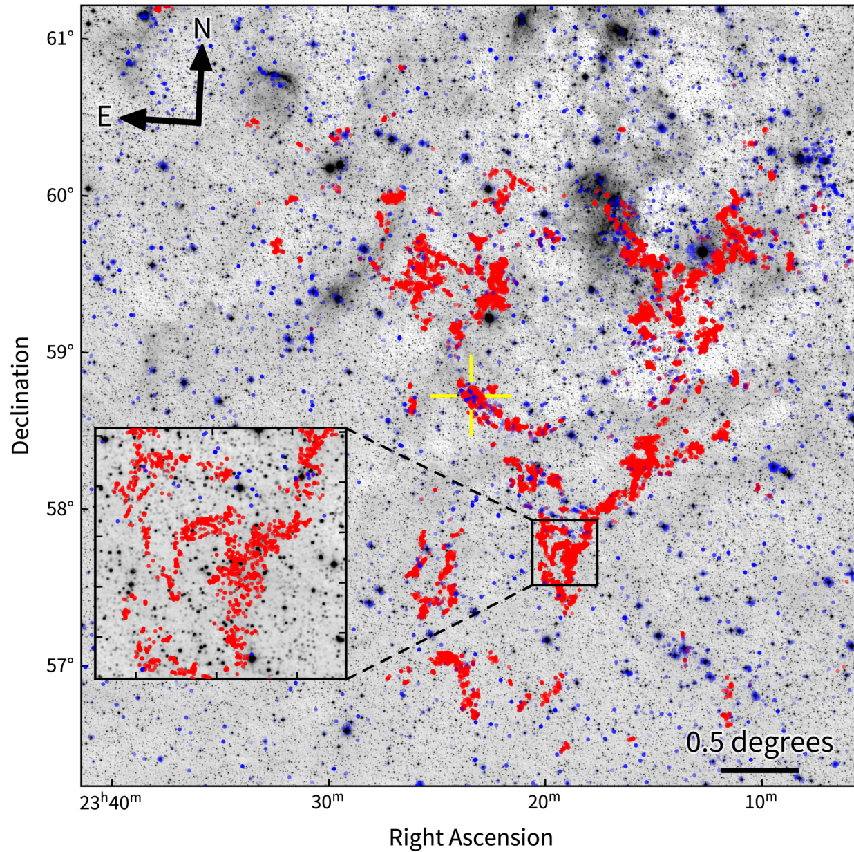
Figure 5. from Justin Vega et al 2026 Astrophys. J. 1008 doi:10.3847/1538-4357/ae96b3 https://dx.doi.org/10.3847/1538-4357/ae96b3 © 2026. The Author(s). Published by the American Astronomical Society.
