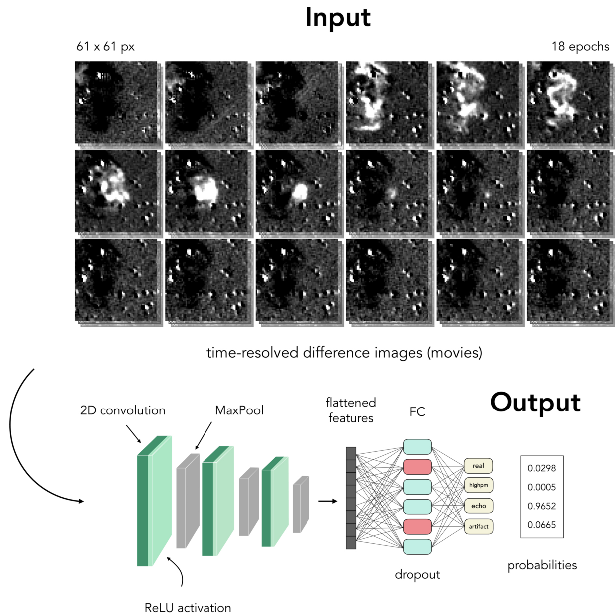
Figure 2. from Justin Vega et al 2026 Astrophys. J. 1008 doi:10.3847/1538-4357/ae96b3 https://dx.doi.org/10.3847/1538-4357/ae96b3 © 2026. The Author(s). Published by the American Astronomical Society.
