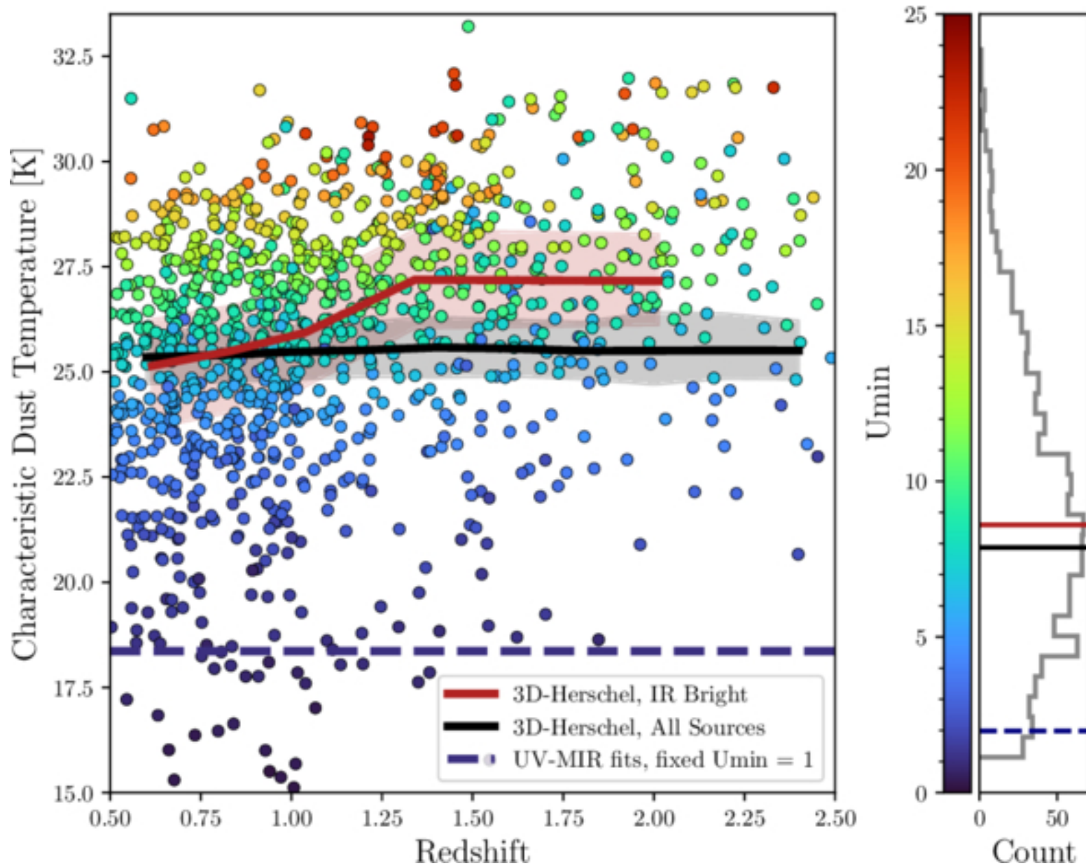
Figure 9. from Seamus McNulty et al 2026 Astrophys. J. 1008 doi:10.3847/1538-4357/ae95f3 https://dx.doi.org/10.3847/1538-4357/ae95f3 © 2026. The Author(s). Published by the American Astronomical Society.
