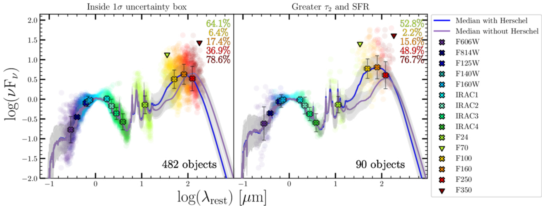
Figure 6. from Seamus McNulty et al 2026 Astrophys. J. 1008 doi:10.3847/1538-4357/ae95f3 https://dx.doi.org/10.3847/1538-4357/ae95f3 © 2026. The Author(s). Published by the American Astronomical Society.
