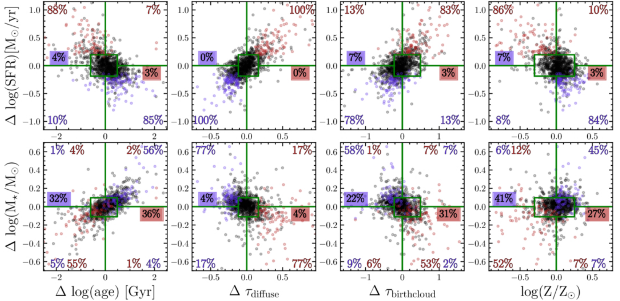
Figure 5. from Seamus McNulty et al 2026 Astrophys. J. 1008 doi:10.3847/1538-4357/ae95f3 https://dx.doi.org/10.3847/1538-4357/ae95f3 © 2026. The Author(s). Published by the American Astronomical Society.
