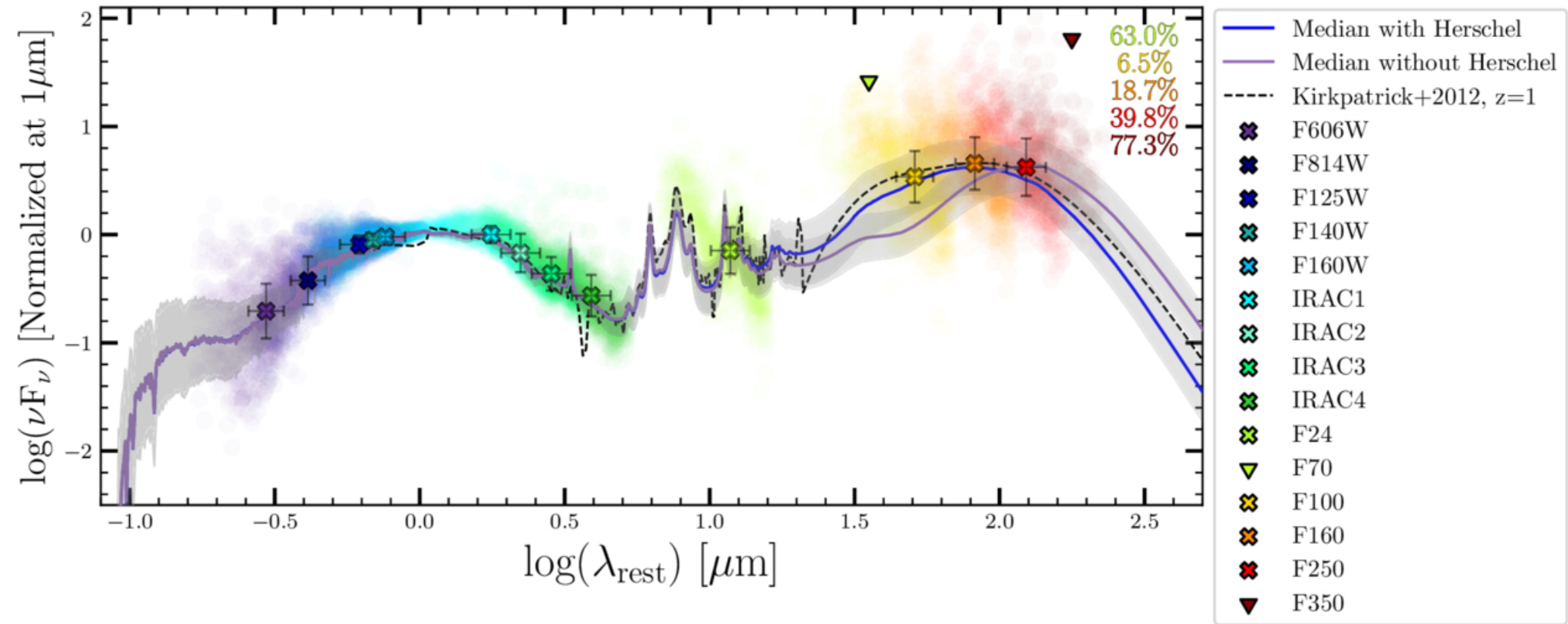
Figure 4. from Seamus McNulty et al 2026 Astrophys. J. 1008 doi:10.3847/1538-4357/ae95f3 https://dx.doi.org/10.3847/1538-4357/ae95f3 © 2026. The Author(s). Published by the American Astronomical Society.
