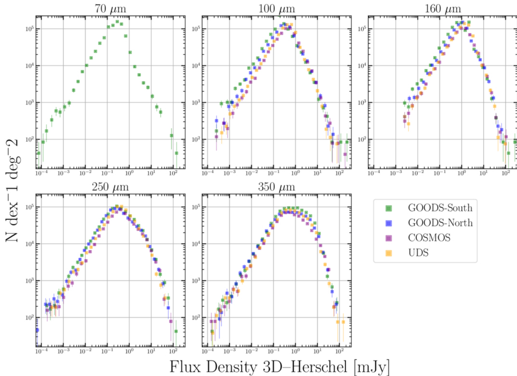
Figure 1. from Seamus McNulty et al 2026 Astrophys. J. 1008 doi:10.3847/1538-4357/ae95f3 https://dx.doi.org/10.3847/1538-4357/ae95f3 © 2026. The Author(s). Published by the American Astronomical Society.
