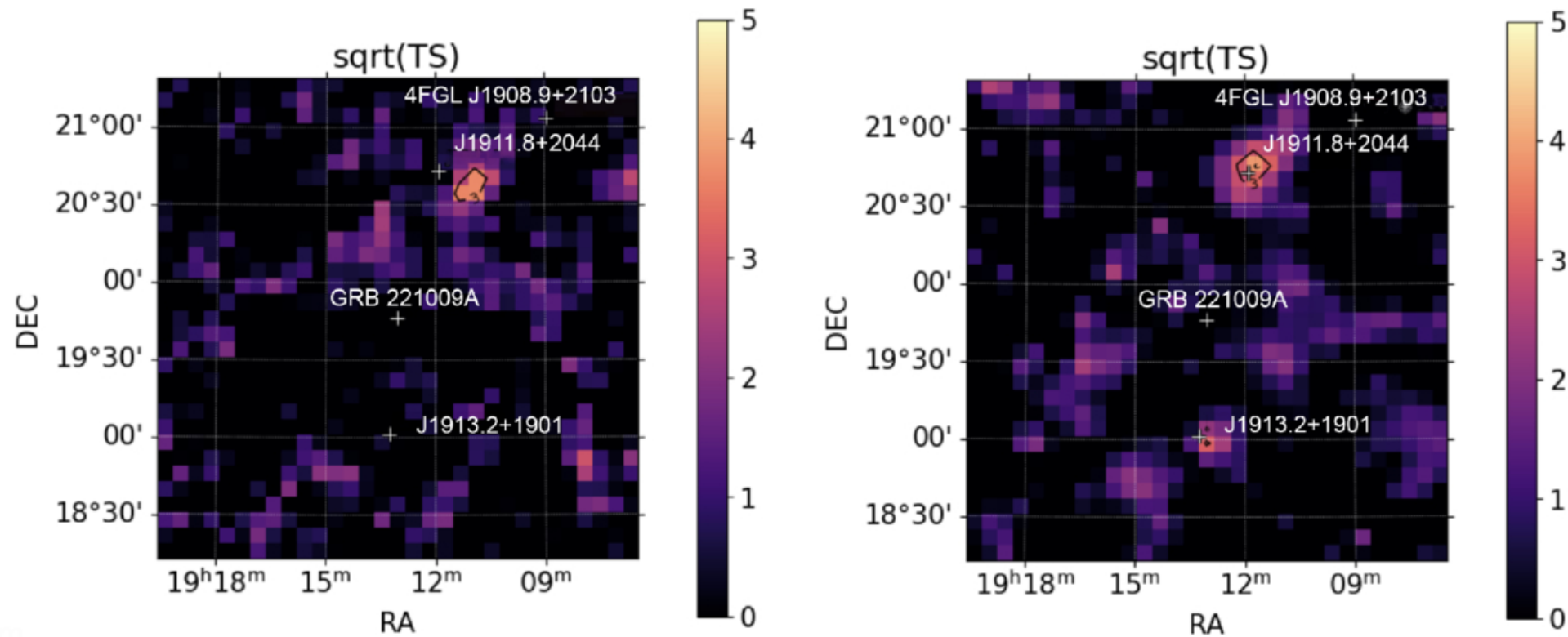
Figure 6. from Saikat Das et al 2026 Astrophys. J. 1008 doi:10.3847/1538-4357/ae9546 https://dx.doi.org/10.3847/1538-4357/ae9546 © 2026. The Author(s). Published by the American Astronomical Society.
