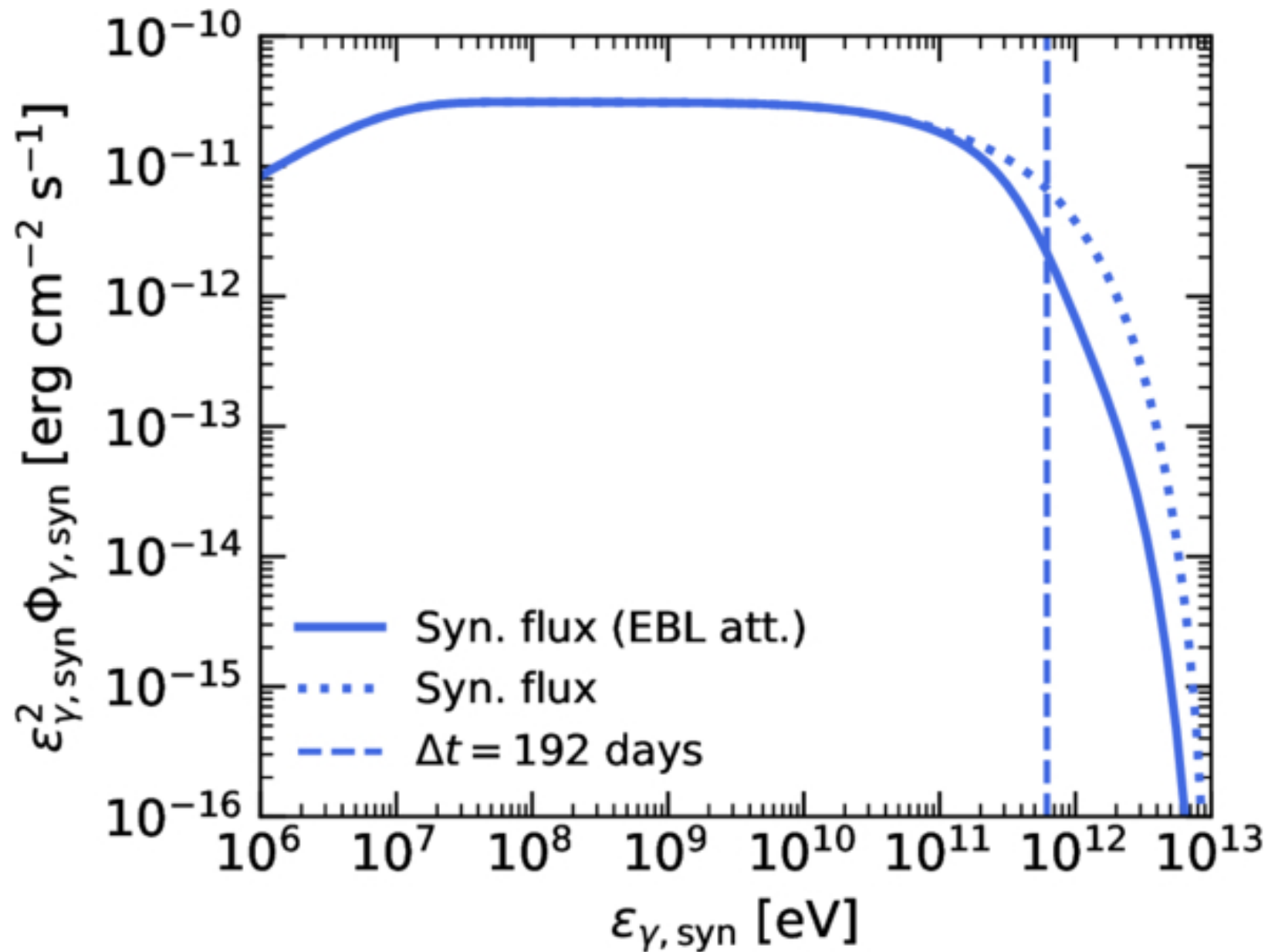
Figure 5. from Saikat Das et al 2026 Astrophys. J. 1008 doi:10.3847/1538-4357/ae9546 https://dx.doi.org/10.3847/1538-4357/ae9546 © 2026. The Author(s). Published by the American Astronomical Society.
