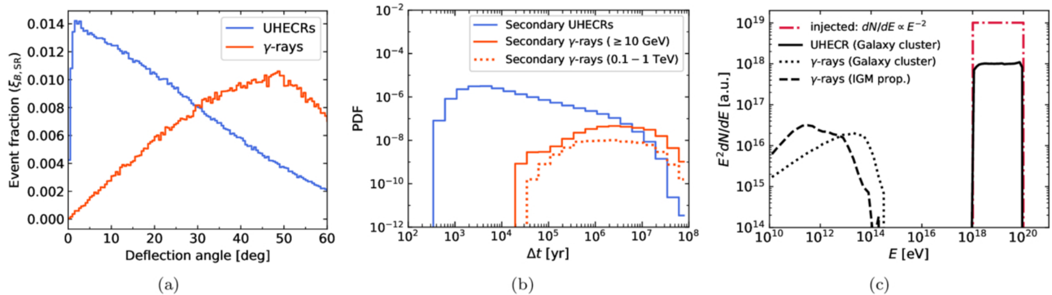
Figure 3. from Saikat Das et al 2026 Astrophys. J. 1008 doi:10.3847/1538-4357/ae9546 https://dx.doi.org/10.3847/1538-4357/ae9546 © 2026. The Author(s). Published by the American Astronomical Society.
