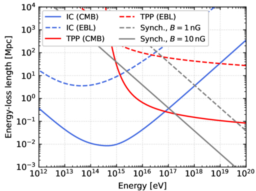
(b) Electrons
