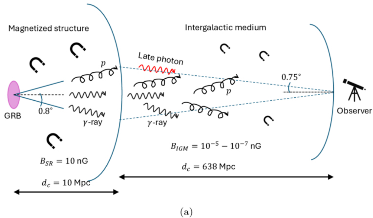
Figure 1. from Saikat Das et al 2026 Astrophys. J. 1008 doi:10.3847/1538-4357/ae9546 https://dx.doi.org/10.3847/1538-4357/ae9546 © 2026. The Author(s). Published by the American Astronomical Society.
