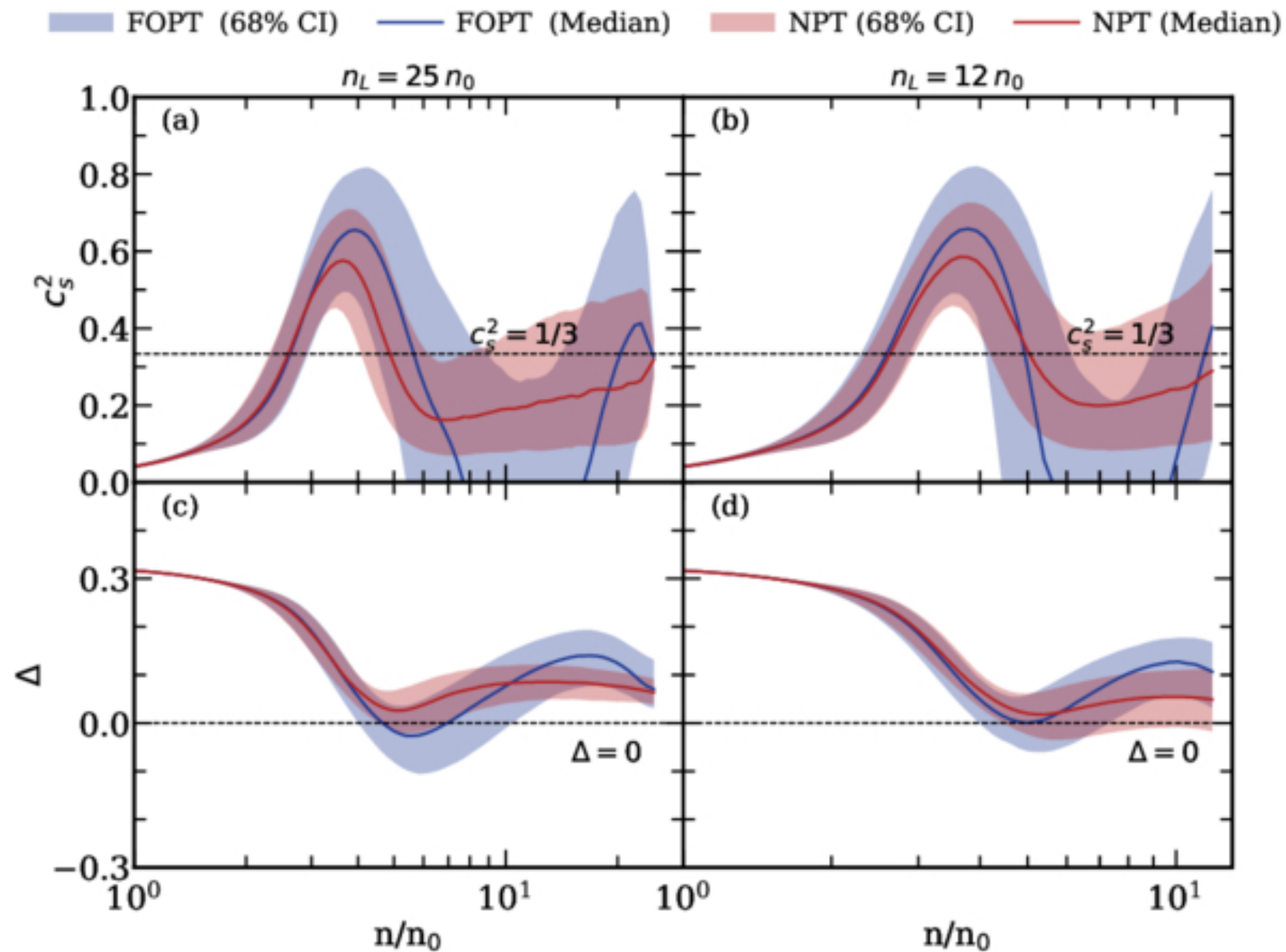
Figure 3. from Zheng Cao and Lie-Wen Chen 2026 Astrophys. J. 1008 doi:10.3847/1538-4357/ae946d https://dx.doi.org/10.3847/1538-4357/ae946d © 2026. The Author(s). Published by the American Astronomical Society.
