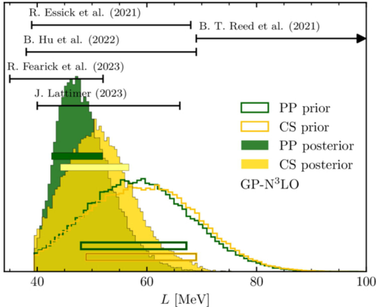
Figure 9. from Melissa Mendes et al 2026 Astrophys. J. 1008 doi:10.3847/1538-4357/ae92f9 https://dx.doi.org/10.3847/1538-4357/ae92f9 © 2026. The Author(s). Published by the American Astronomical Society.
