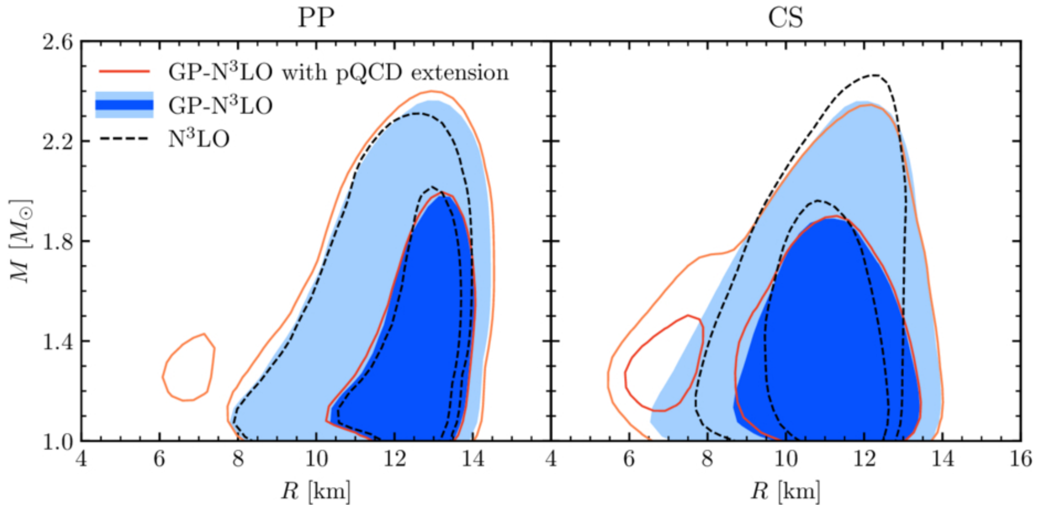
Figure 3. from Melissa Mendes et al 2026 Astrophys. J. 1008 doi:10.3847/1538-4357/ae92f9 https://dx.doi.org/10.3847/1538-4357/ae92f9 © 2026. The Author(s). Published by the American Astronomical Society.
