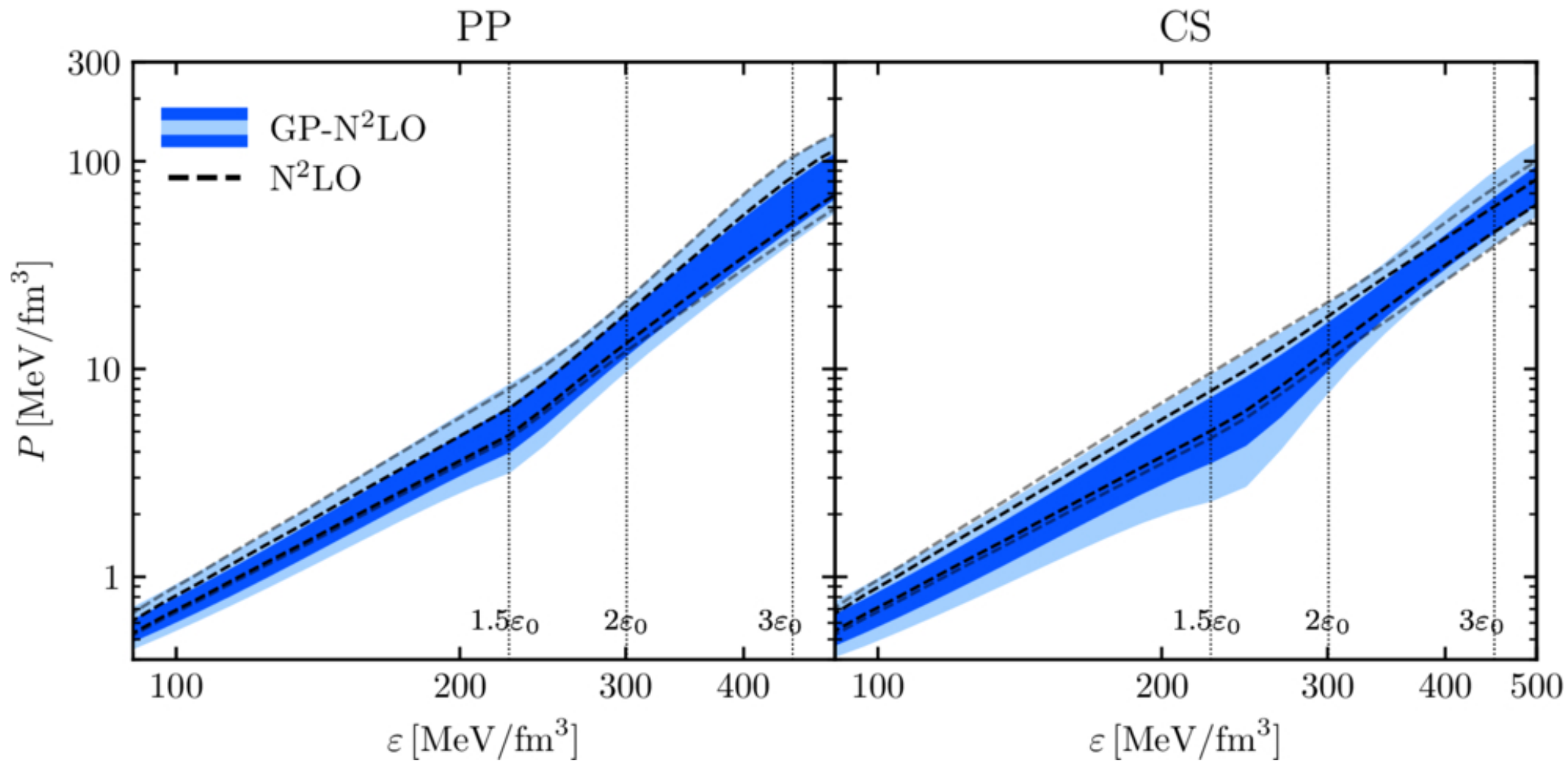
Figure 15. from Melissa Mendes et al 2026 Astrophys. J. 1008 doi:10.3847/1538-4357/ae92f9 https://dx.doi.org/10.3847/1538-4357/ae92f9 © 2026. The Author(s). Published by the American Astronomical Society.
