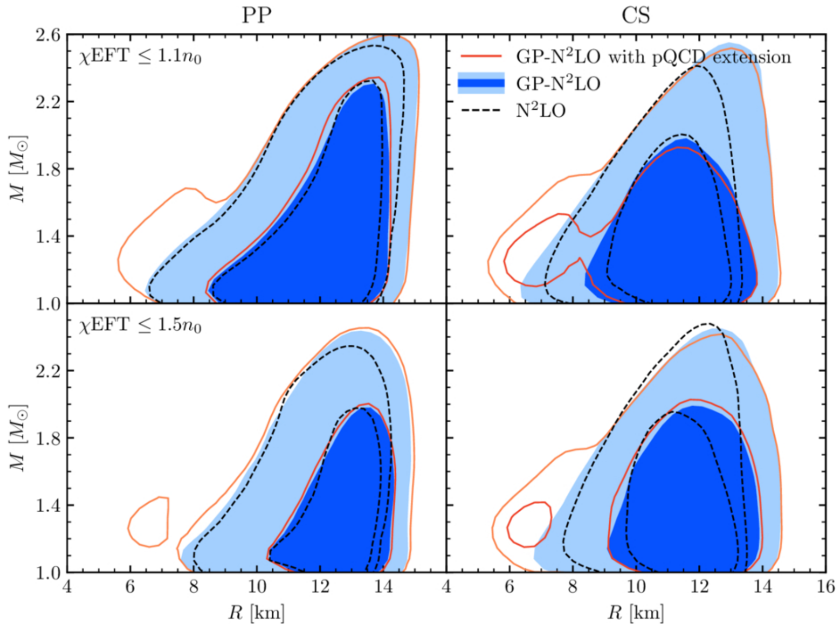
Figure 12. from Melissa Mendes et al 2026 Astrophys. J. 1008 doi:10.3847/1538-4357/ae92f9 https://dx.doi.org/10.3847/1538-4357/ae92f9 © 2026. The Author(s). Published by the American Astronomical Society.
