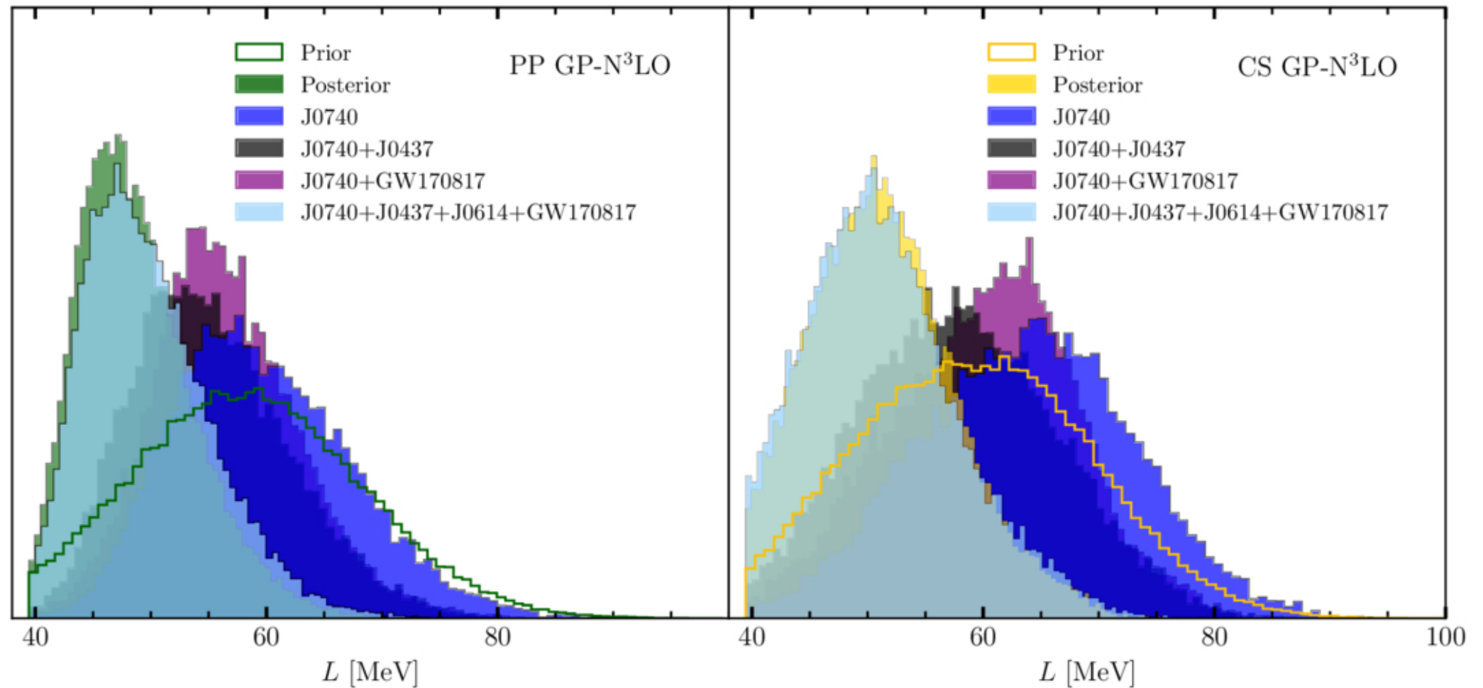
Figure 11. from Melissa Mendes et al 2026 Astrophys. J. 1008 doi:10.3847/1538-4357/ae92f9 https://dx.doi.org/10.3847/1538-4357/ae92f9 © 2026. The Author(s). Published by the American Astronomical Society.
