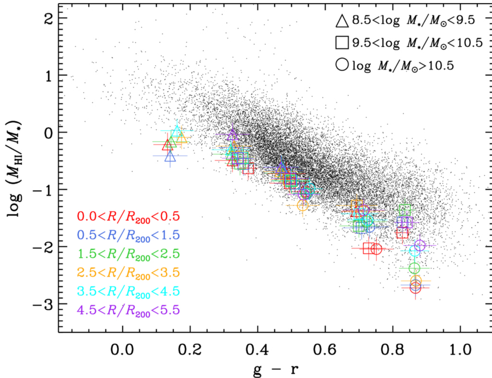
Figure 7. from Cheng Cheng et al 2026 Astrophys. J. 1009 doi:10.3847/1538-4357/ae928e https://dx.doi.org/10.3847/1538-4357/ae928e © 2026. The Author(s). Published by the American Astronomical Society.
