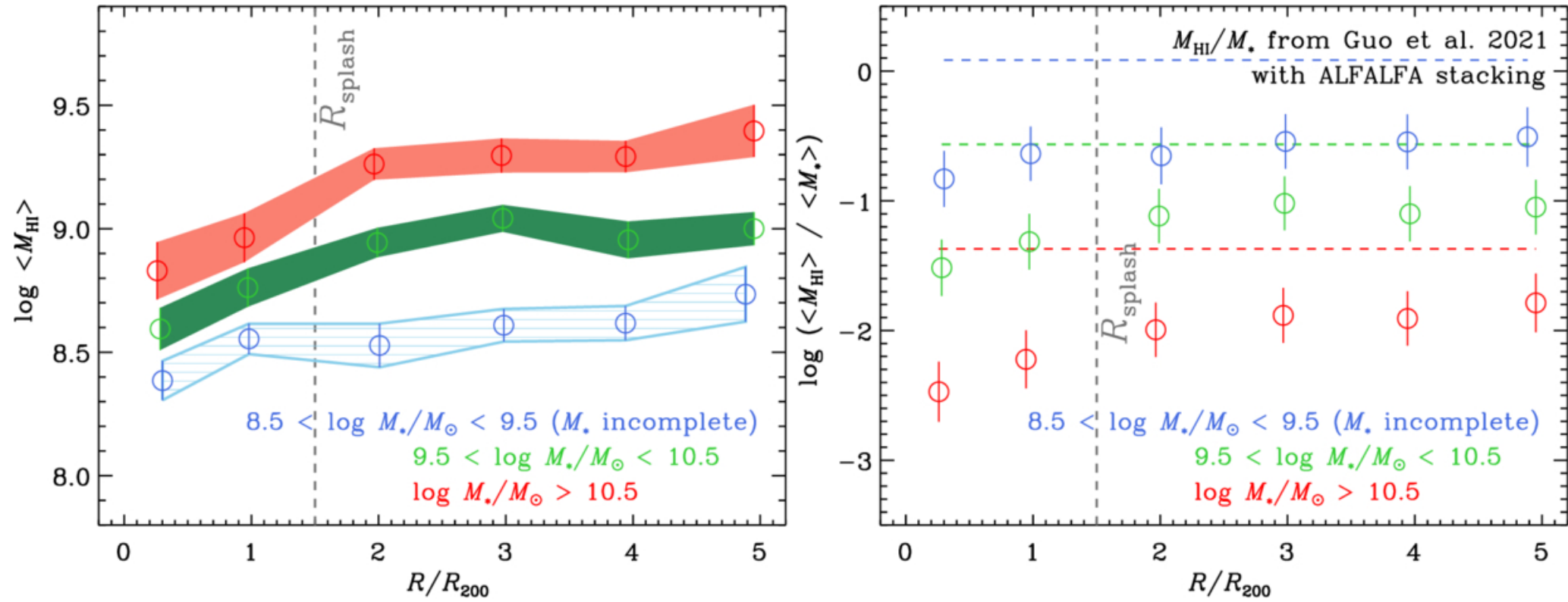
Figure 5. from Cheng Cheng et al 2026 Astrophys. J. 1009 doi:10.3847/1538-4357/ae928e https://dx.doi.org/10.3847/1538-4357/ae928e © 2026. The Author(s). Published by the American Astronomical Society.
