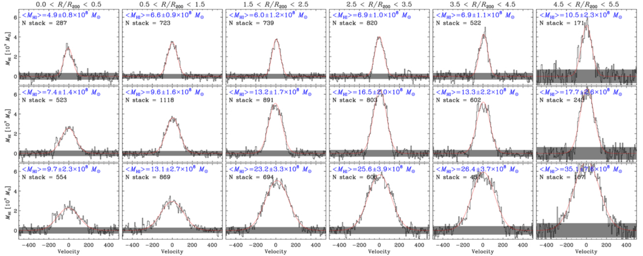
Figure 4. from Cheng Cheng et al 2026 Astrophys. J. 1009 doi:10.3847/1538-4357/ae928e https://dx.doi.org/10.3847/1538-4357/ae928e © 2026. The Author(s). Published by the American Astronomical Society.
