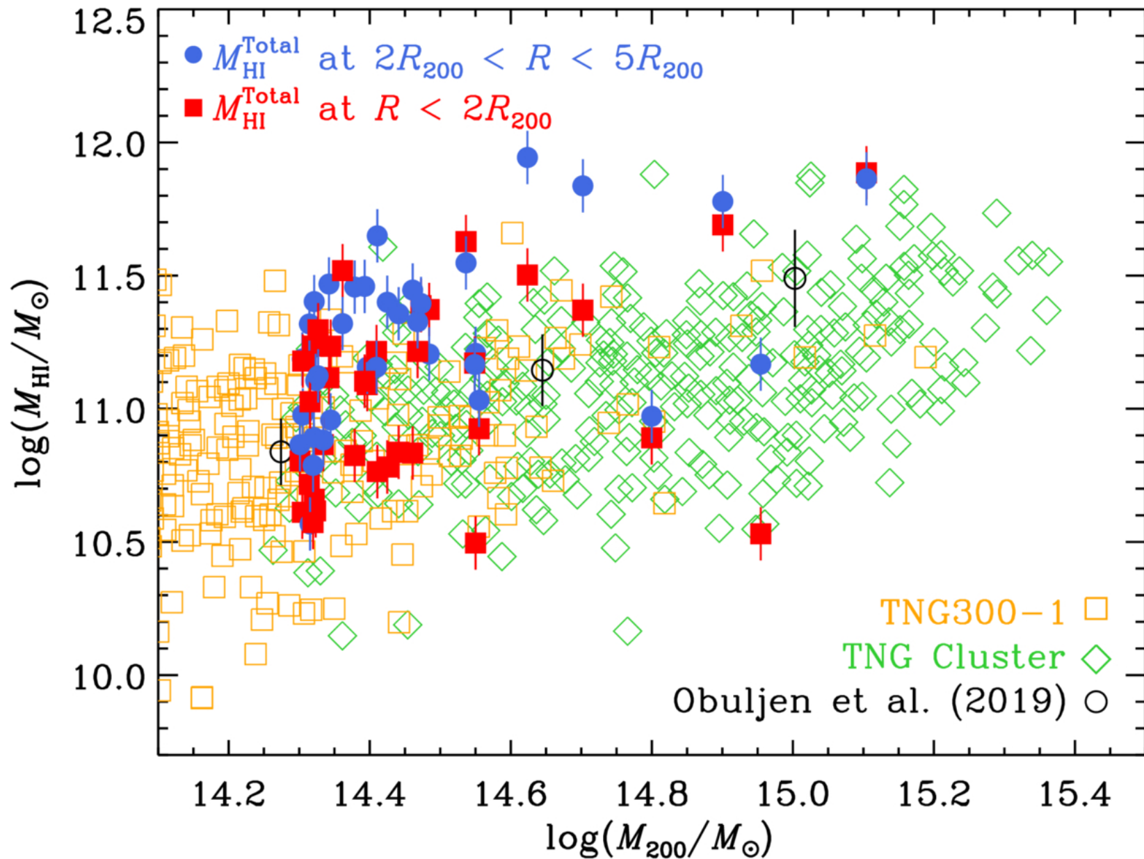
Figure 11. from Cheng Cheng et al 2026 Astrophys. J. 1009 doi:10.3847/1538-4357/ae928e https://dx.doi.org/10.3847/1538-4357/ae928e © 2026. The Author(s). Published by the American Astronomical Society.
