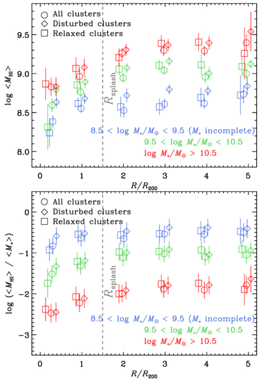
Figure 10. from Cheng Cheng et al 2026 Astrophys. J. 1009 doi:10.3847/1538-4357/ae928e https://dx.doi.org/10.3847/1538-4357/ae928e © 2026. The Author(s). Published by the American Astronomical Society.
