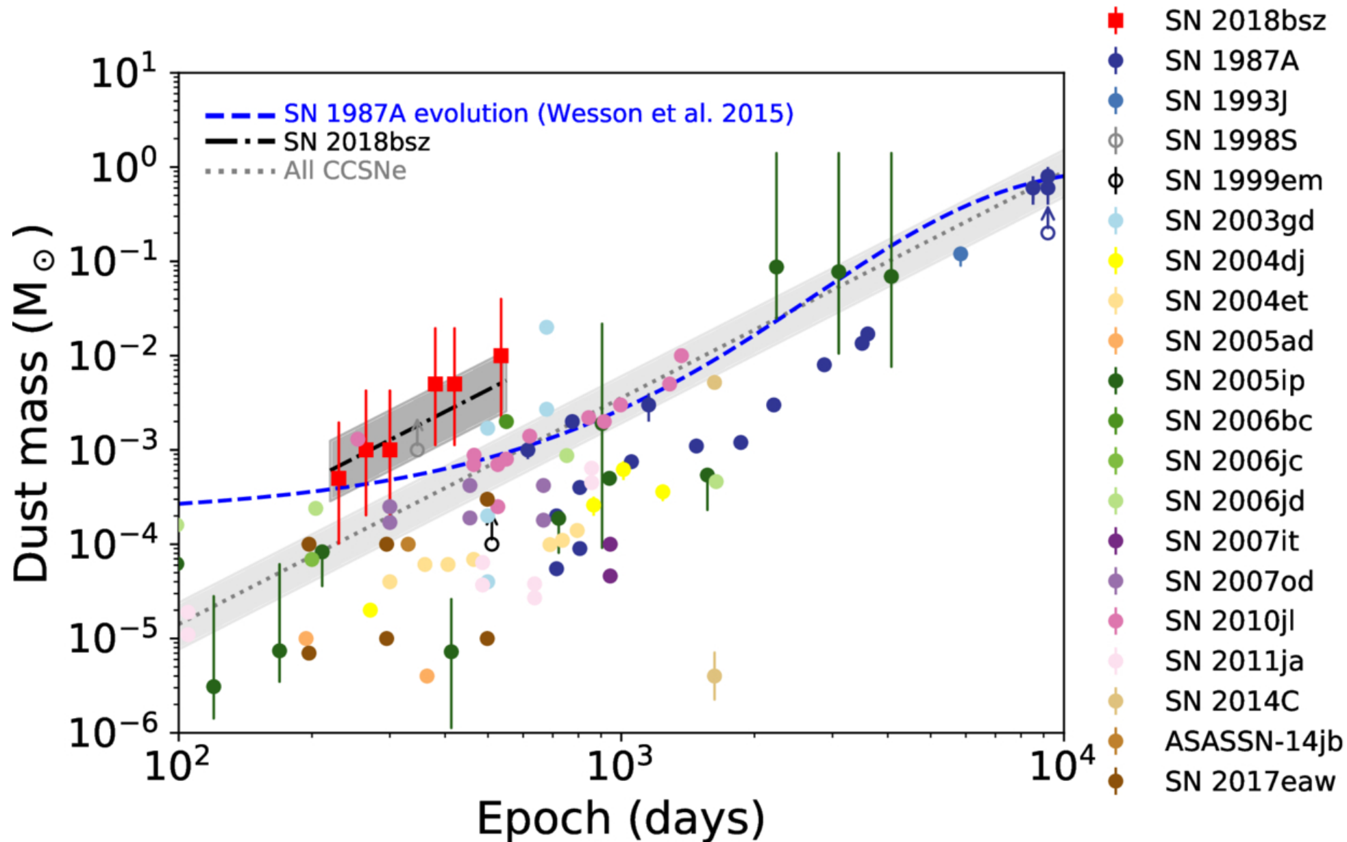
Figure 9. from T.-W. Chen et al 2026 Astrophys. J. 1009 doi:10.3847/1538-4357/ae91e7 https://dx.doi.org/10.3847/1538-4357/ae91e7 © 2026. The Author(s). Published by the American Astronomical Society.
