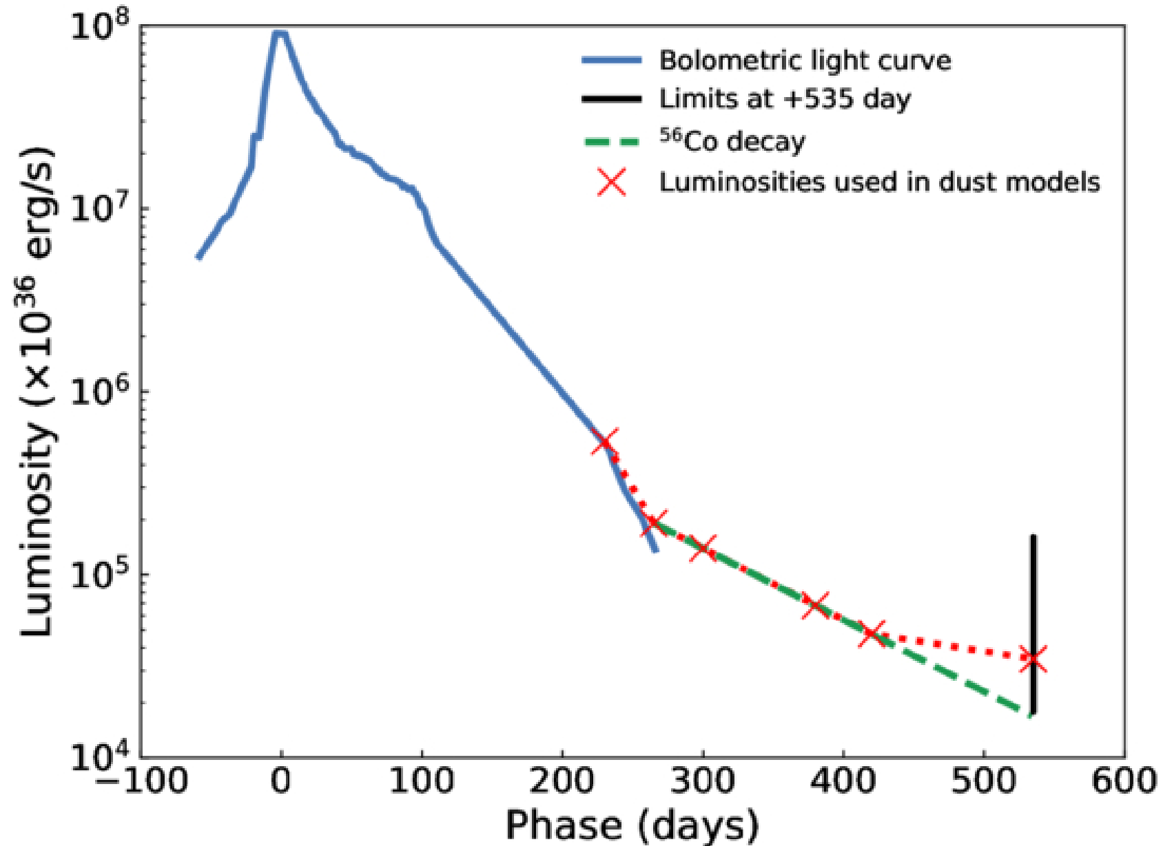
Figure 7. from T.-W. Chen et al 2026 Astrophys. J. 1009 doi:10.3847/1538-4357/ae91e7 https://dx.doi.org/10.3847/1538-4357/ae91e7 © 2026. The Author(s). Published by the American Astronomical Society.
