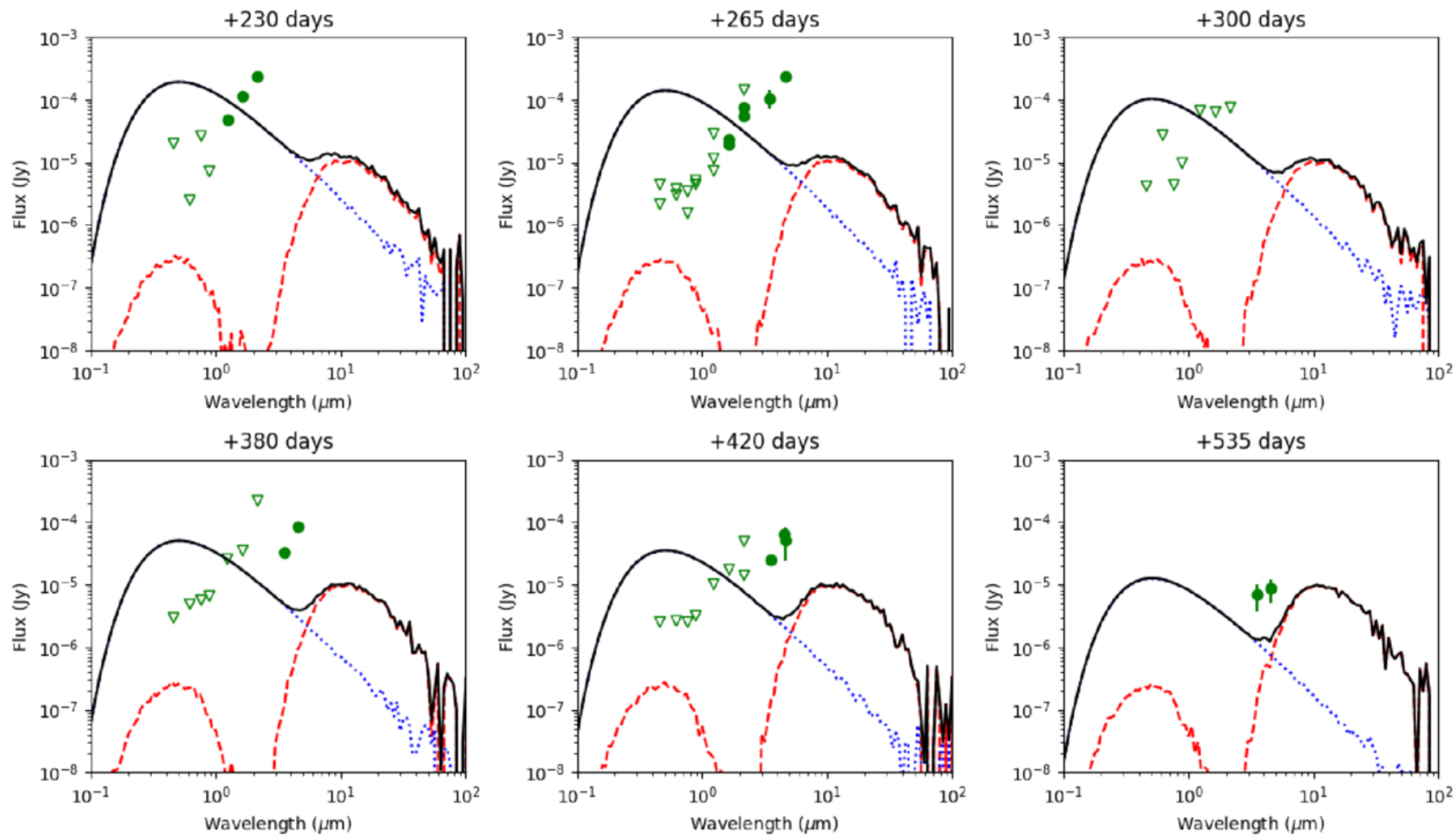
Figure 4. from T.-W. Chen et al 2026 Astrophys. J. 1009 doi:10.3847/1538-4357/ae91e7 https://dx.doi.org/10.3847/1538-4357/ae91e7 © 2026. The Author(s). Published by the American Astronomical Society.
