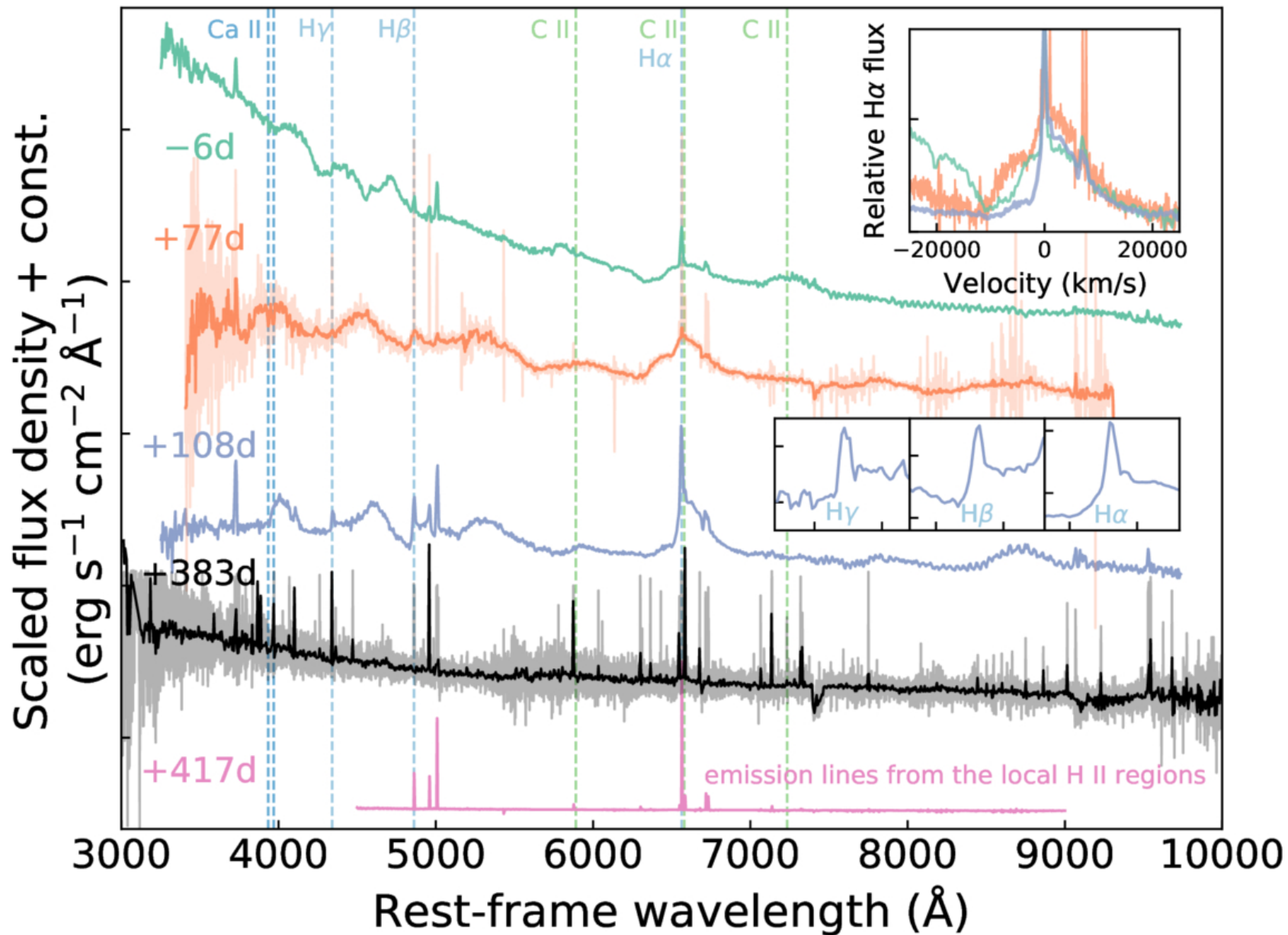
Figure 2. from T.-W. Chen et al 2026 Astrophys. J. 1009 doi:10.3847/1538-4357/ae91e7 https://dx.doi.org/10.3847/1538-4357/ae91e7 © 2026. The Author(s). Published by the American Astronomical Society.
