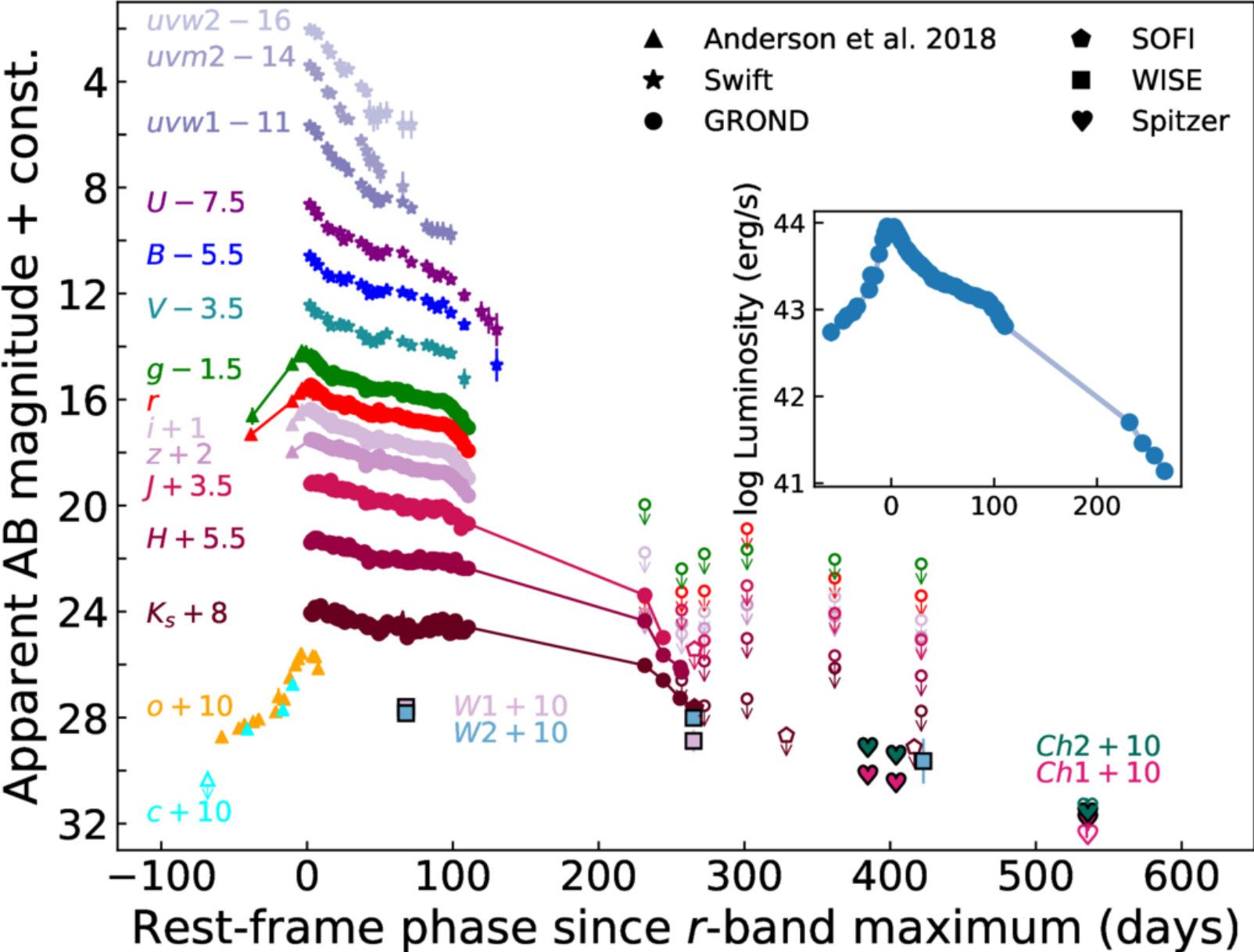
Figure 1. from T.-W. Chen et al 2026 Astrophys. J. 1009 doi:10.3847/1538-4357/ae91e7 https://dx.doi.org/10.3847/1538-4357/ae91e7 © 2026. The Author(s). Published by the American Astronomical Society.
