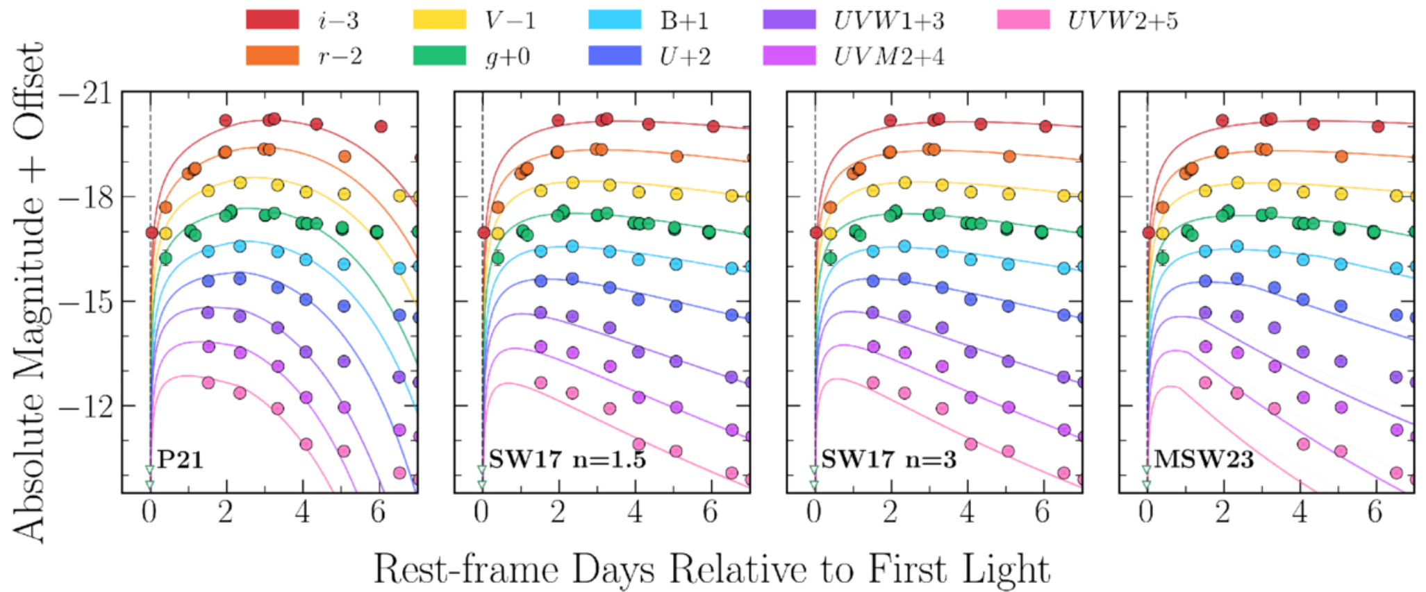
Figure 8. from R. J. Yete et al 2026 Astrophys. J. 1009 doi:10.3847/1538-4357/ae91e3 https://dx.doi.org/10.3847/1538-4357/ae91e3 © 2026. The Author(s). Published by the American Astronomical Society.
