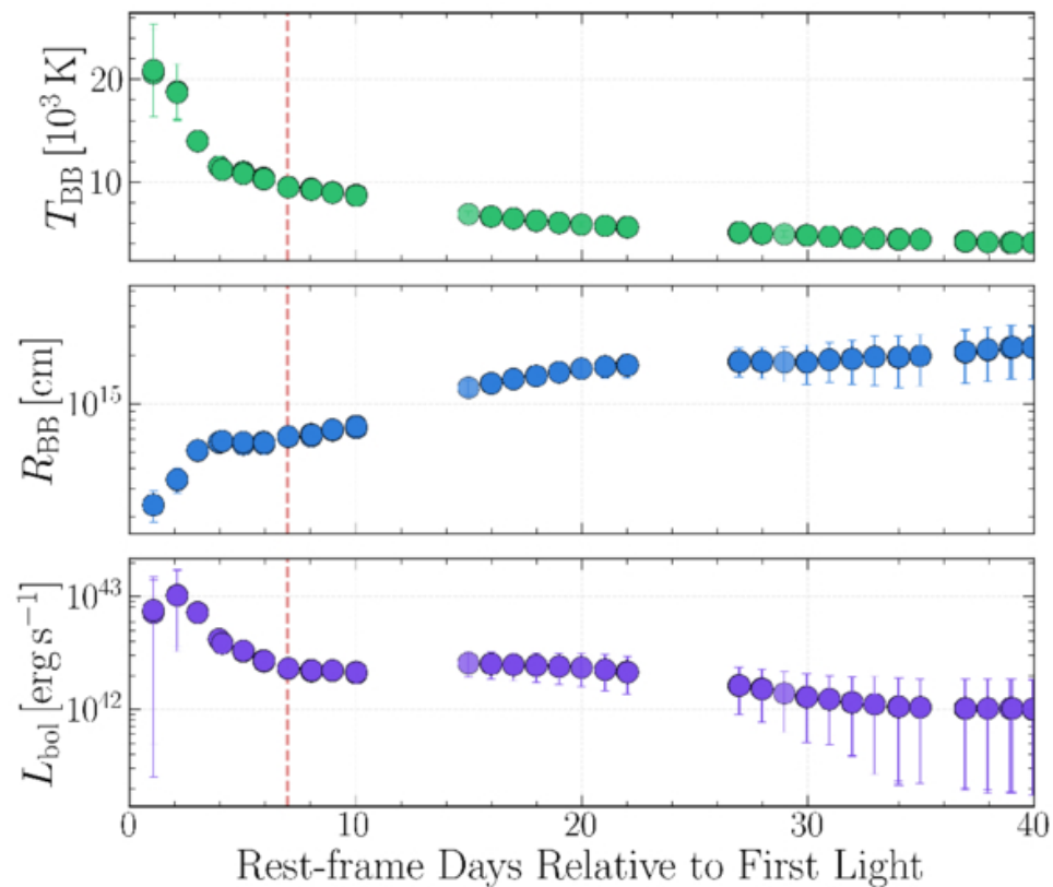
Figure 6. from R. J. Yete et al 2026 Astrophys. J. 1009 doi:10.3847/1538-4357/ae91e3 https://dx.doi.org/10.3847/1538-4357/ae91e3 © 2026. The Author(s). Published by the American Astronomical Society.
