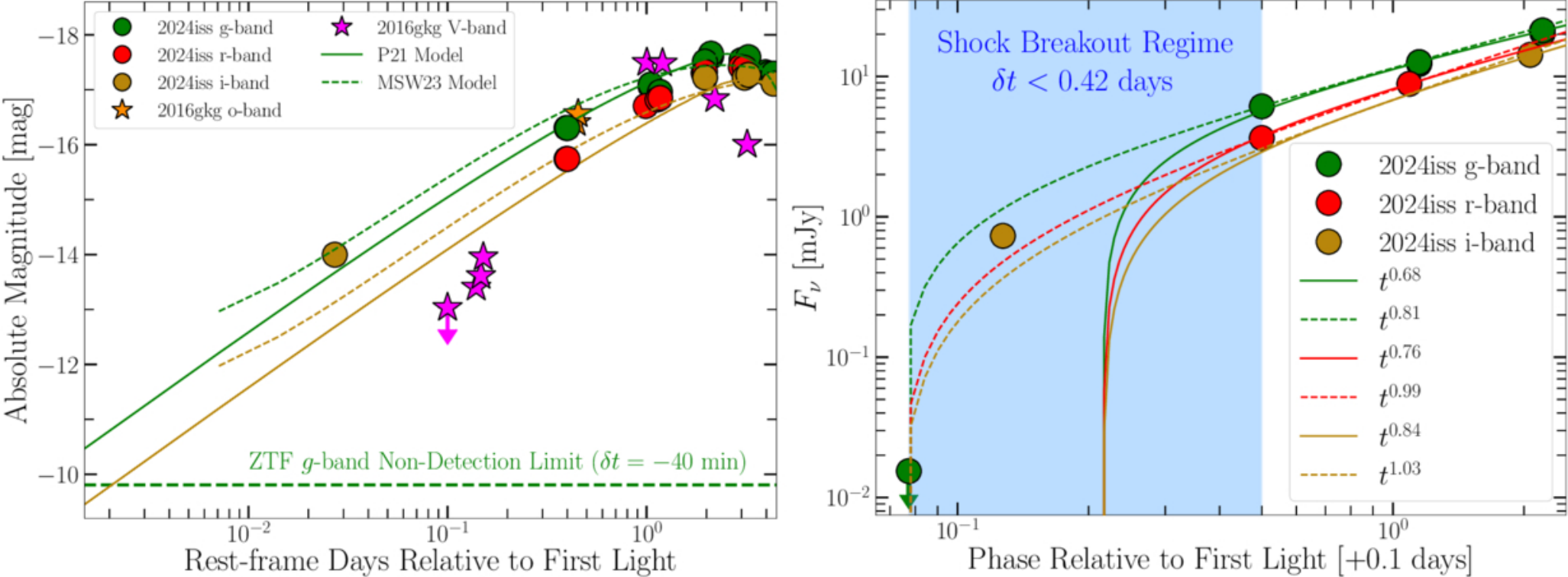
Figure 5. from R. J. Yete et al 2026 Astrophys. J. 1009 doi:10.3847/1538-4357/ae91e3 https://dx.doi.org/10.3847/1538-4357/ae91e3 © 2026. The Author(s). Published by the American Astronomical Society.
