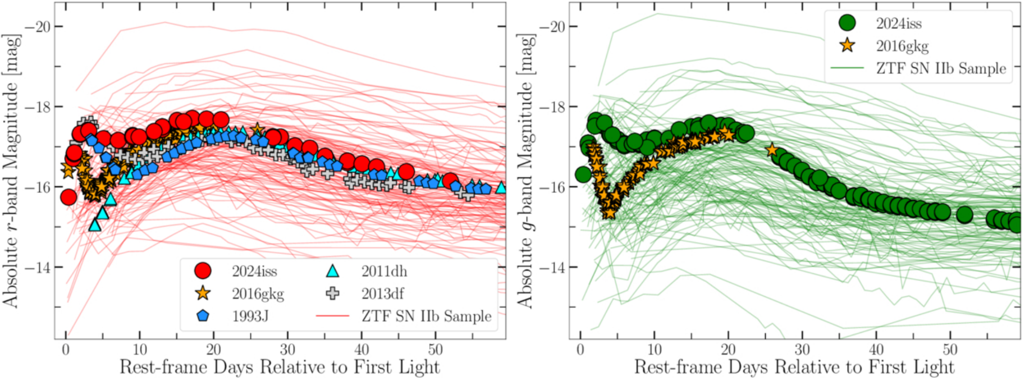
Figure 4. from R. J. Yete et al 2026 Astrophys. J. 1009 doi:10.3847/1538-4357/ae91e3 https://dx.doi.org/10.3847/1538-4357/ae91e3 © 2026. The Author(s). Published by the American Astronomical Society.
