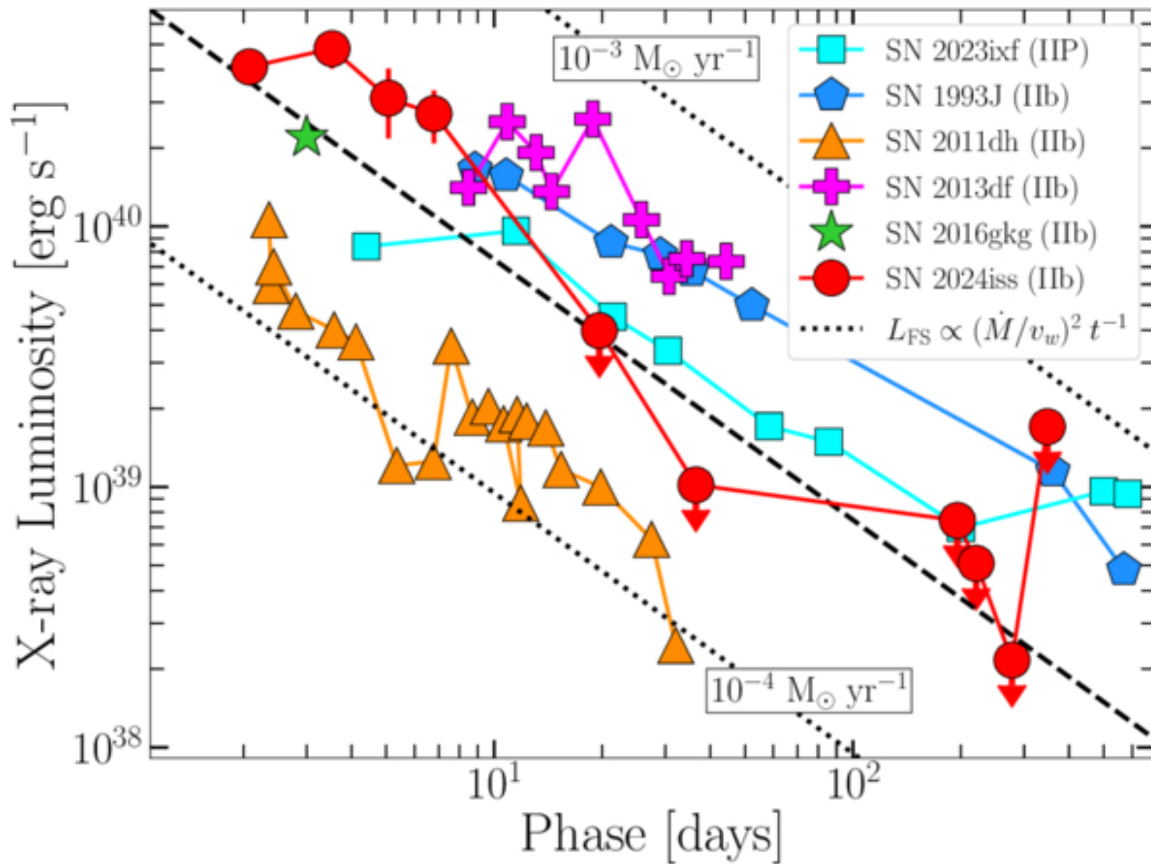
Figure 3. from R. J. Yete et al 2026 Astrophys. J. 1009 doi:10.3847/1538-4357/ae91e3 https://dx.doi.org/10.3847/1538-4357/ae91e3 © 2026. The Author(s). Published by the American Astronomical Society.
