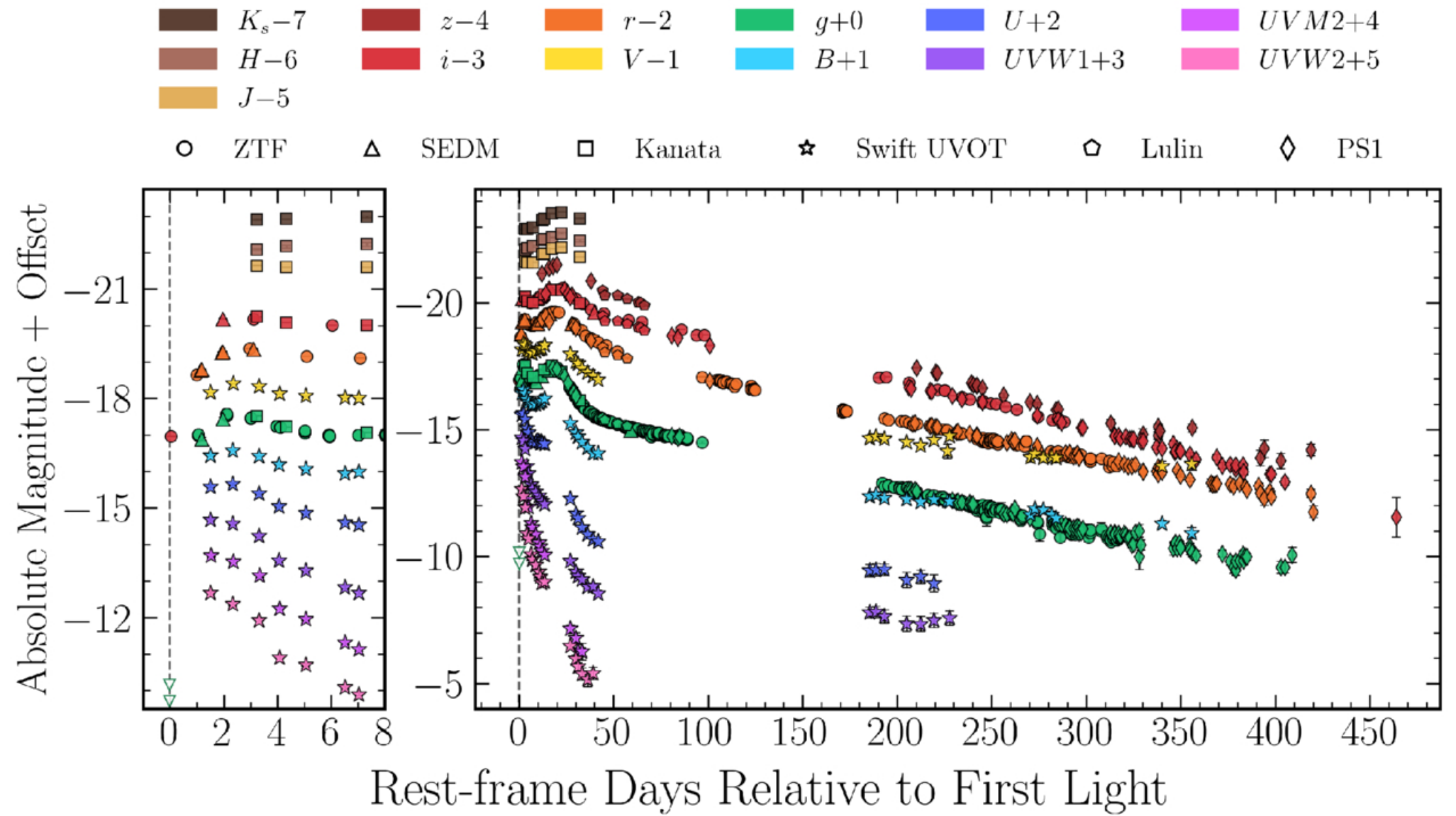
Figure 2. from R. J. Yete et al 2026 Astrophys. J. 1009 doi:10.3847/1538-4357/ae91e3 https://dx.doi.org/10.3847/1538-4357/ae91e3 © 2026. The Author(s). Published by the American Astronomical Society.
