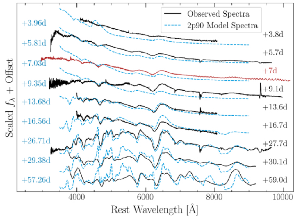
Figure 14. from R. J. Yete et al 2026 Astrophys. J. 1009 doi:10.3847/1538-4357/ae91e3 https://dx.doi.org/10.3847/1538-4357/ae91e3 © 2026. The Author(s). Published by the American Astronomical Society.
