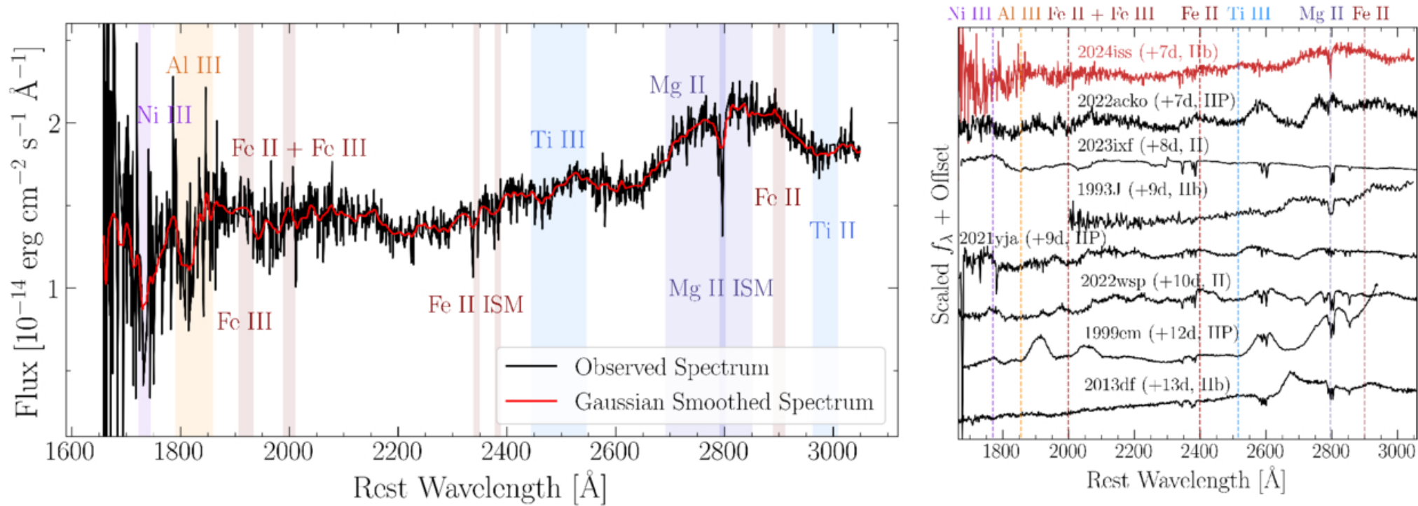
Figure 12. from R. J. Yete et al 2026 Astrophys. J. 1009 doi:10.3847/1538-4357/ae91e3 https://dx.doi.org/10.3847/1538-4357/ae91e3 © 2026. The Author(s). Published by the American Astronomical Society.
