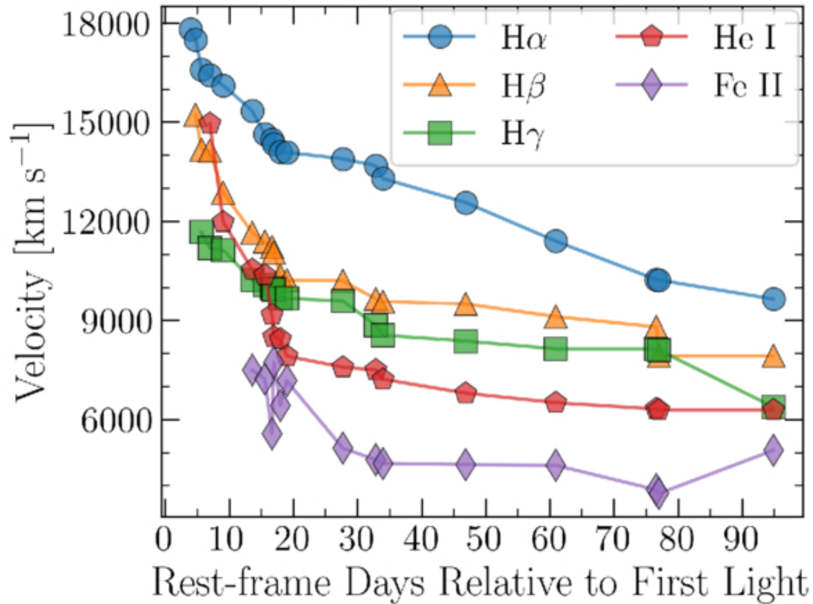
Figure 10. from R. J. Yete et al 2026 Astrophys. J. 1009 doi:10.3847/1538-4357/ae91e3 https://dx.doi.org/10.3847/1538-4357/ae91e3 © 2026. The Author(s). Published by the American Astronomical Society.
