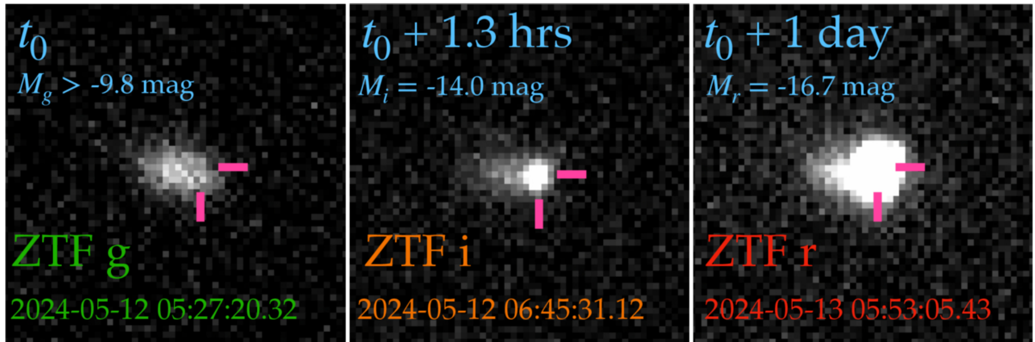
Figure 1. from R. J. Yete et al 2026 Astrophys. J. 1009 doi:10.3847/1538-4357/ae91e3 https://dx.doi.org/10.3847/1538-4357/ae91e3 © 2026. The Author(s). Published by the American Astronomical Society.
