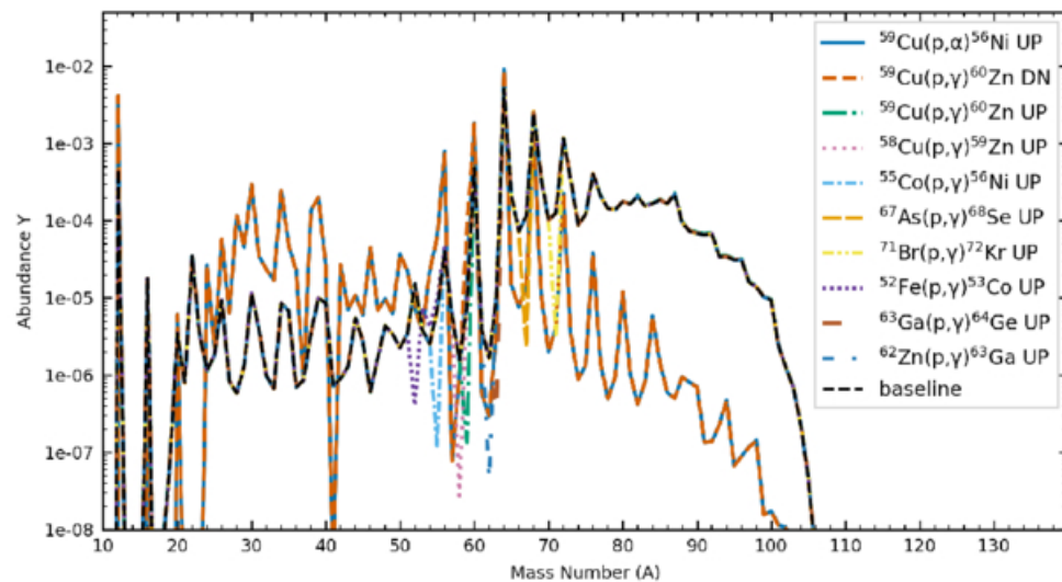
Figure 7. from I. Sultana et al 2026 Astrophys. J. 1009 doi:10.3847/1538-4357/ae9163 https://dx.doi.org/10.3847/1538-4357/ae9163 © 2026. The Author(s). Published by the American Astronomical Society.
