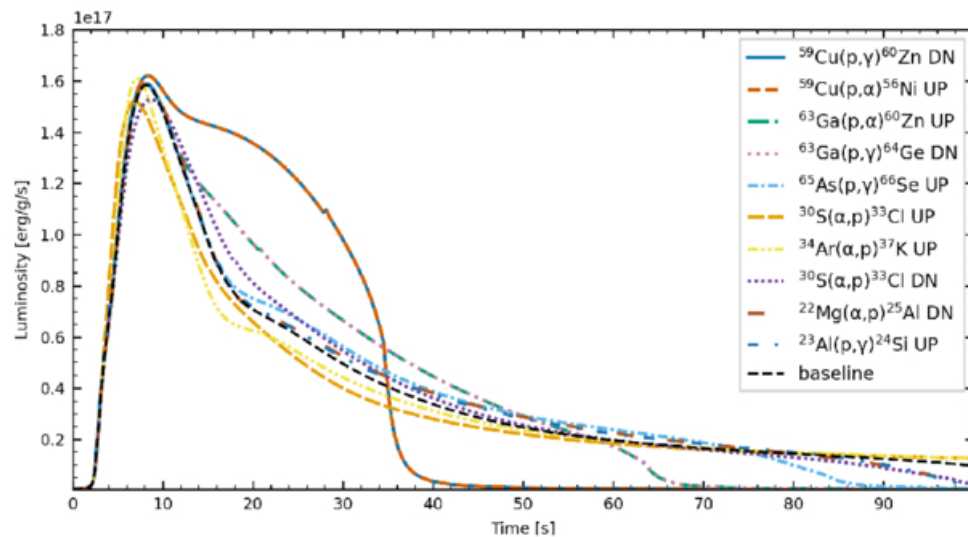
Figure 6. from I. Sultana et al 2026 Astrophys. J. 1009 doi:10.3847/1538-4357/ae9163 https://dx.doi.org/10.3847/1538-4357/ae9163 © 2026. The Author(s). Published by the American Astronomical Society.
