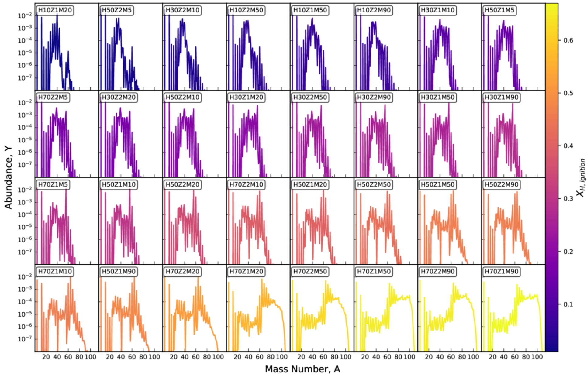
Figure 5. from I. Sultana et al 2026 Astrophys. J. 1009 doi:10.3847/1538-4357/ae9163 https://dx.doi.org/10.3847/1538-4357/ae9163 © 2026. The Author(s). Published by the American Astronomical Society.
