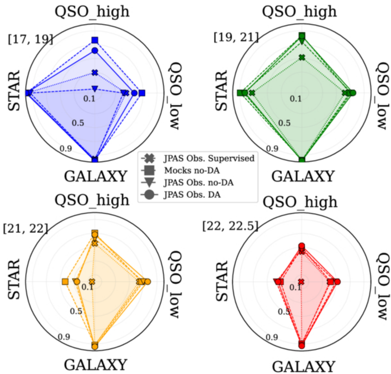
Figure 8. from Daniel López-Cano et al 2026 Astrophys. J. 1008 doi:10.3847/1538-4357/ae915c https://dx.doi.org/10.3847/1538-4357/ae915c © 2026. The Author(s). Published by the American Astronomical Society.
