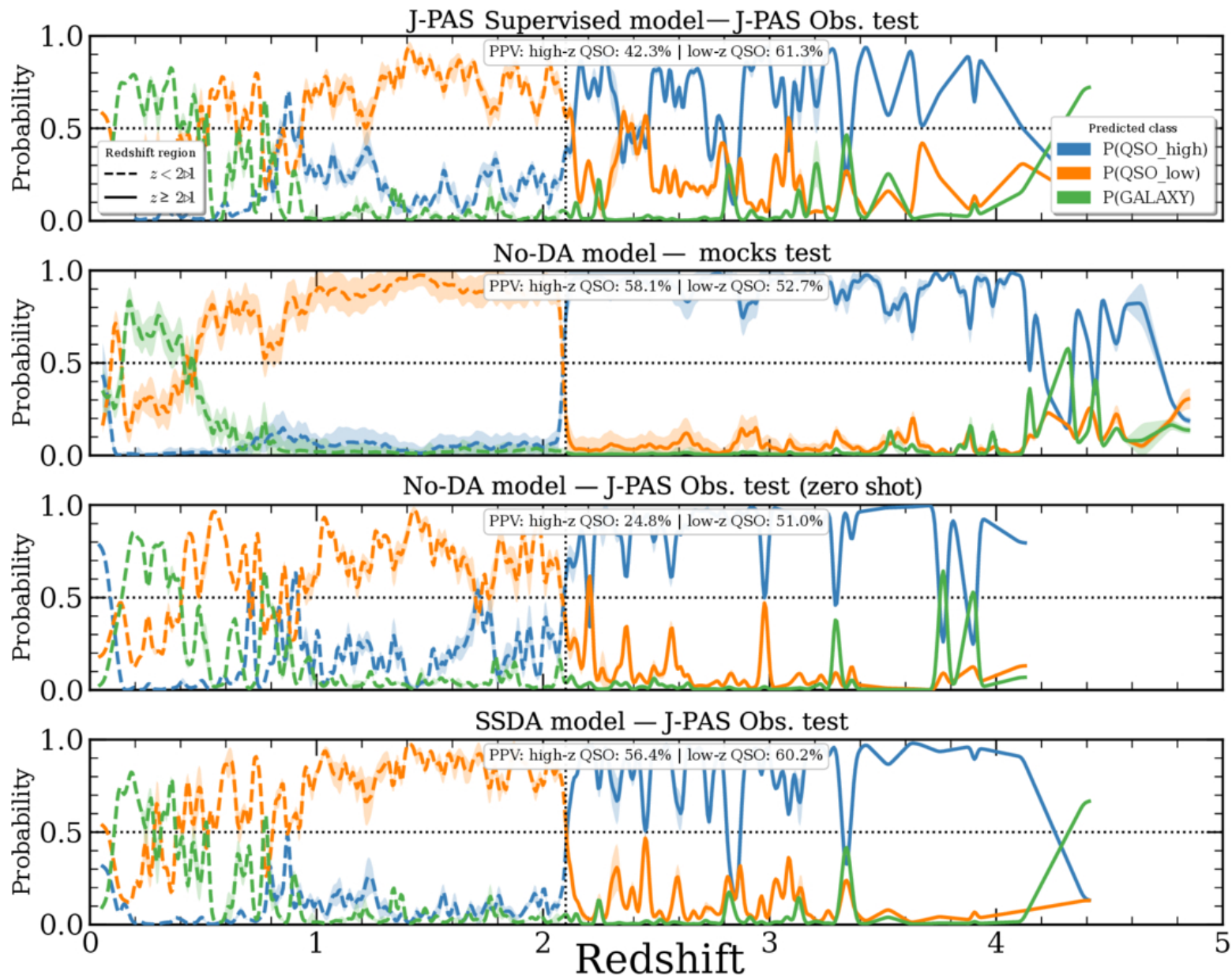
Figure 5. from Daniel López-Cano et al 2026 Astrophys. J. 1008 doi:10.3847/1538-4357/ae915c https://dx.doi.org/10.3847/1538-4357/ae915c © 2026. The Author(s). Published by the American Astronomical Society.
