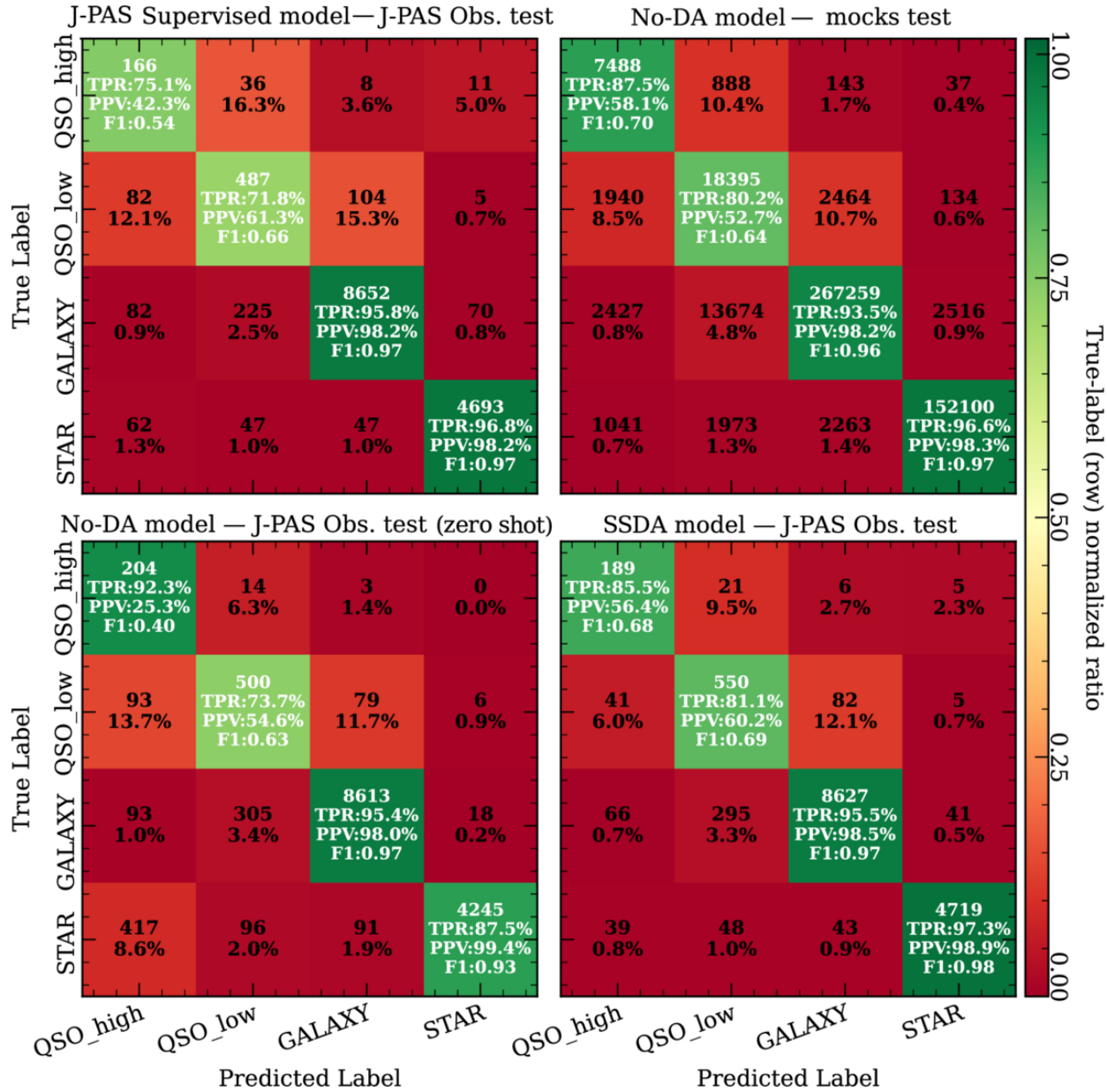
Figure 3. from Daniel López-Cano et al 2026 Astrophys. J. 1008 doi:10.3847/1538-4357/ae915c https://dx.doi.org/10.3847/1538-4357/ae915c © 2026. The Author(s). Published by the American Astronomical Society.
