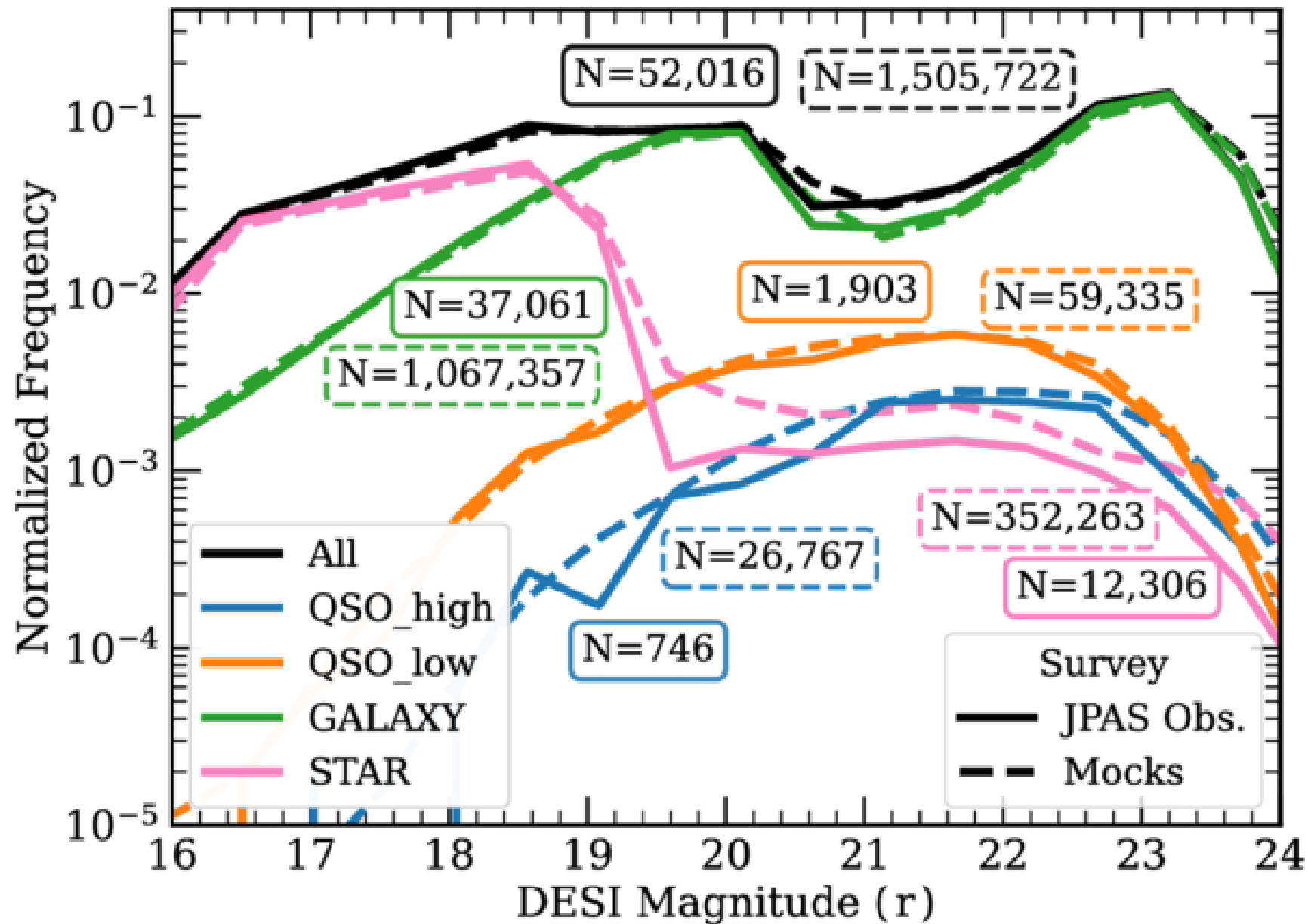
Figure 2. from Daniel López-Cano et al 2026 Astrophys. J. 1008 doi:10.3847/1538-4357/ae915c https://dx.doi.org/10.3847/1538-4357/ae915c © 2026. The Author(s). Published by the American Astronomical Society.
