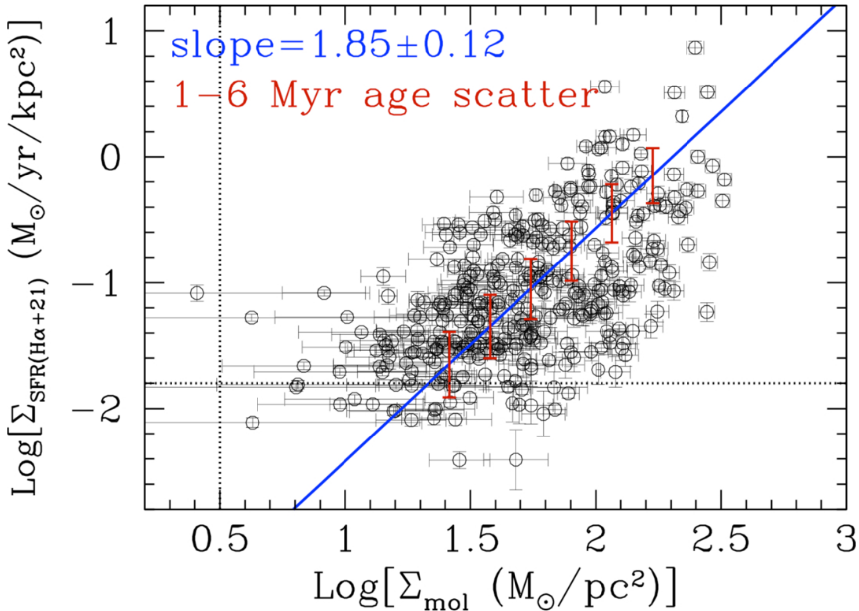
Figure 9. from Daniela Calzetti et al 2026 Astrophys. J. 1008 doi:10.3847/1538-4357/ae915b https://dx.doi.org/10.3847/1538-4357/ae915b © 2026. The Author(s). Published by the American Astronomical Society.
