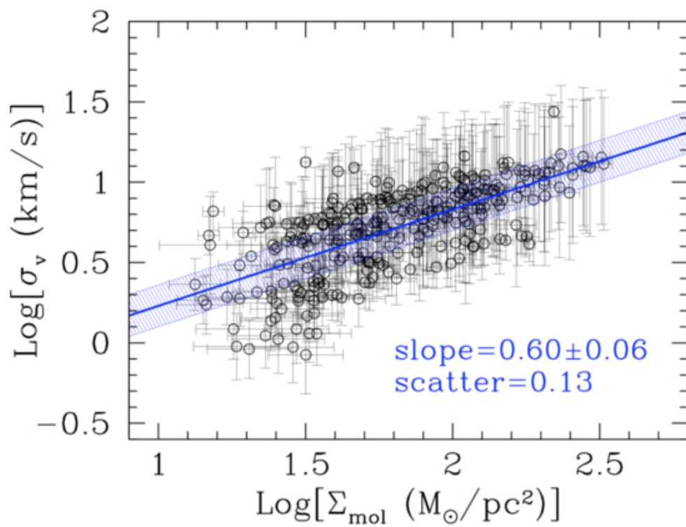
Figure 8. from Daniela Calzetti et al 2026 Astrophys. J. 1008 doi:10.3847/1538-4357/ae915b https://dx.doi.org/10.3847/1538-4357/ae915b © 2026. The Author(s). Published by the American Astronomical Society.
