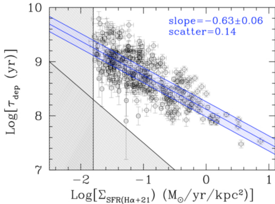
Figure 7. from Daniela Calzetti et al 2026 Astrophys. J. 1008 doi:10.3847/1538-4357/ae915b https://dx.doi.org/10.3847/1538-4357/ae915b © 2026. The Author(s). Published by the American Astronomical Society.
