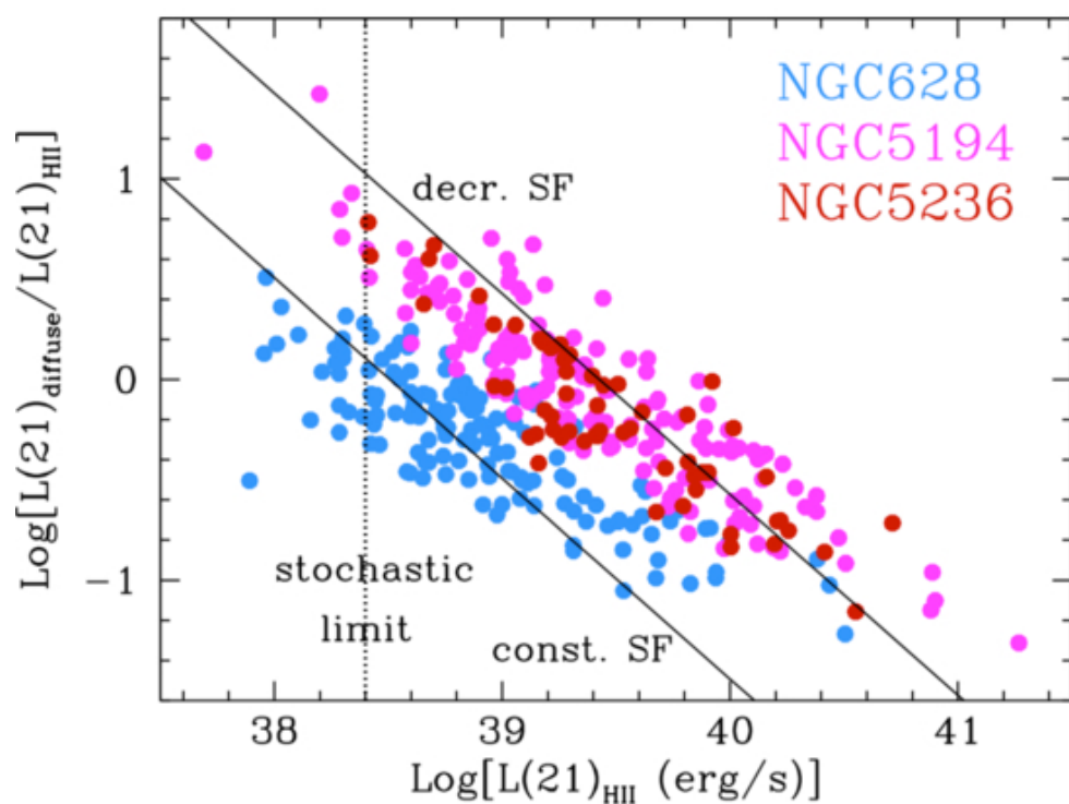
Figure 3. from Daniela Calzetti et al 2026 Astrophys. J. 1008 doi:10.3847/1538-4357/ae915b https://dx.doi.org/10.3847/1538-4357/ae915b © 2026. The Author(s). Published by the American Astronomical Society.
