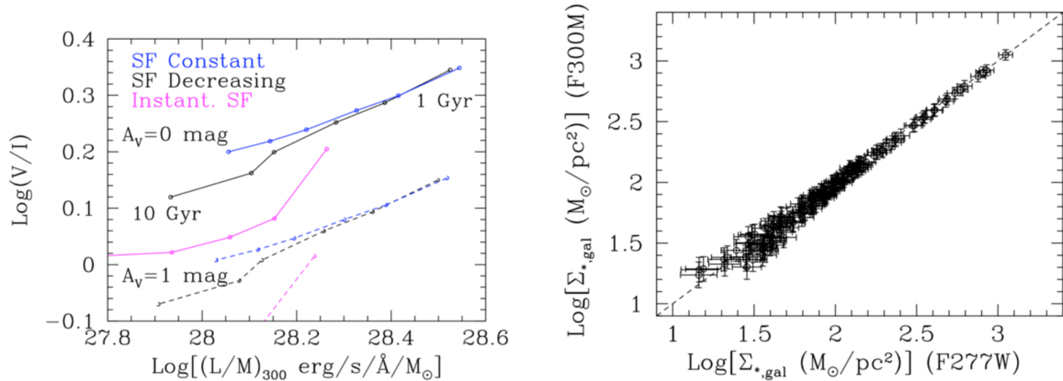
Figure 14. from Daniela Calzetti et al 2026 Astrophys. J. 1008 doi:10.3847/1538-4357/ae915b https://dx.doi.org/10.3847/1538-4357/ae915b © 2026. The Author(s). Published by the American Astronomical Society.
